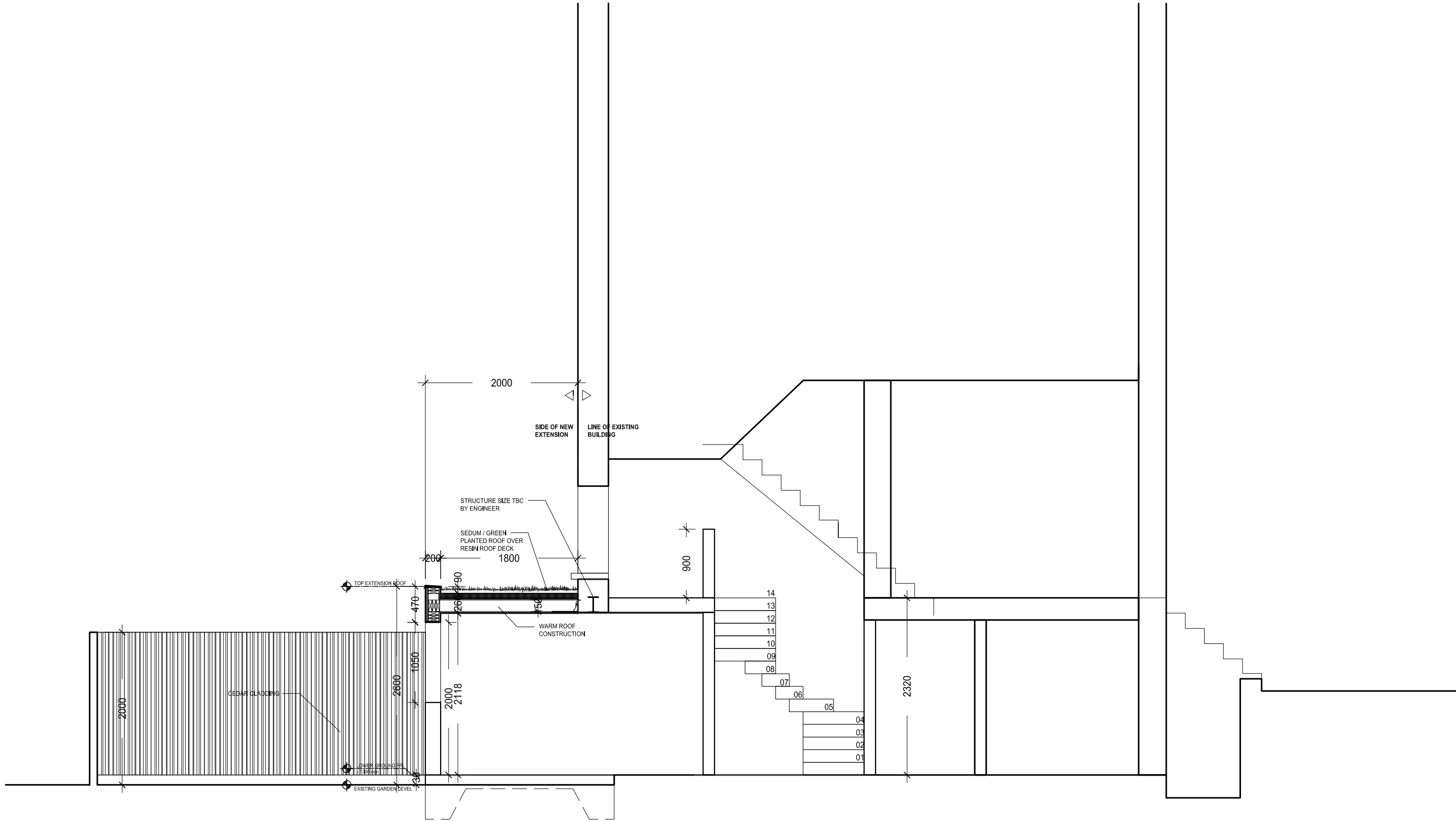
1 PROPOSED LONG SECTION SCALE: 1:50 @ A3
