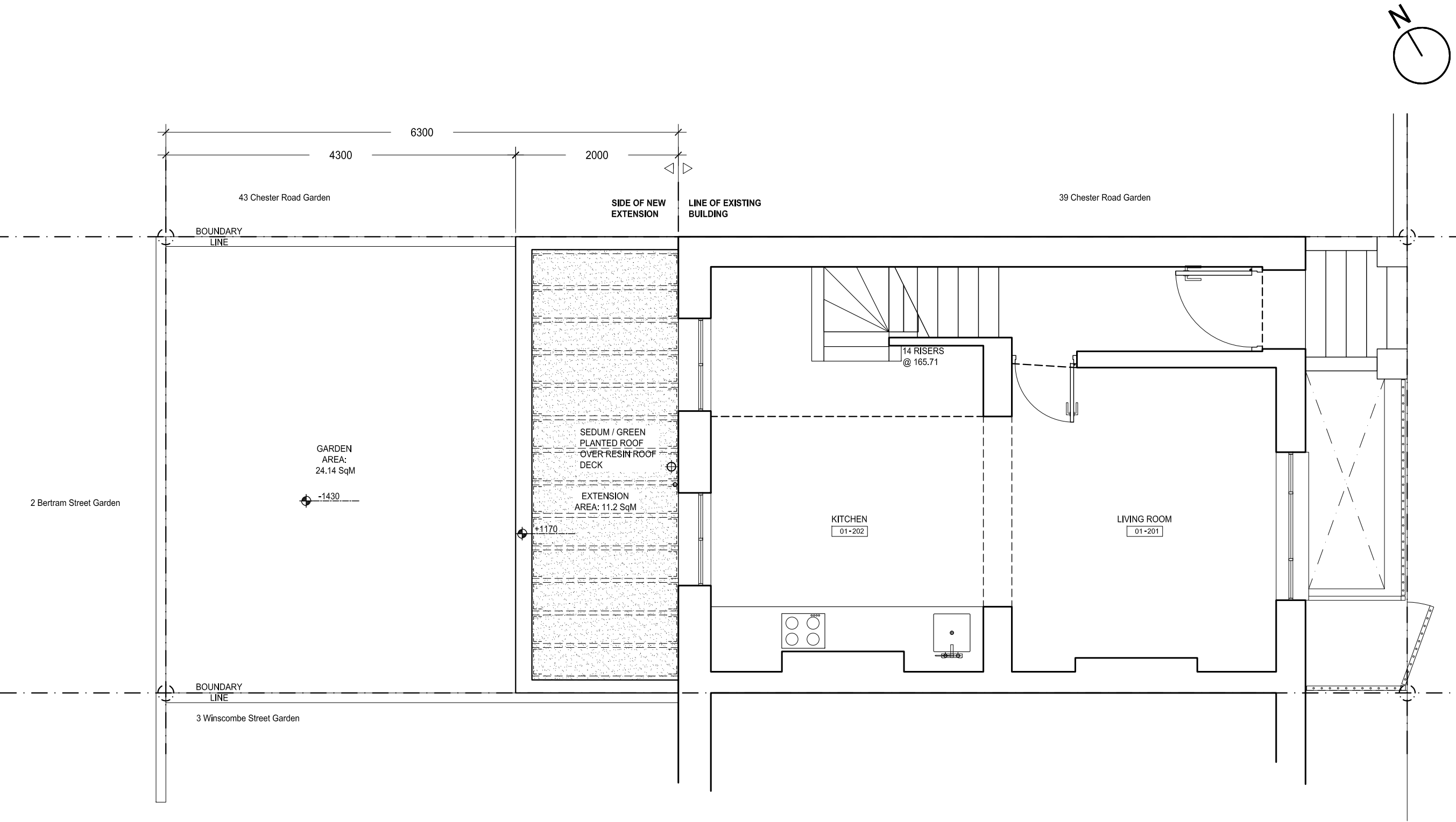
1 PROPOSED UPPER GROUND FLOOR PLAN SCALE: 1:50 @ A3
