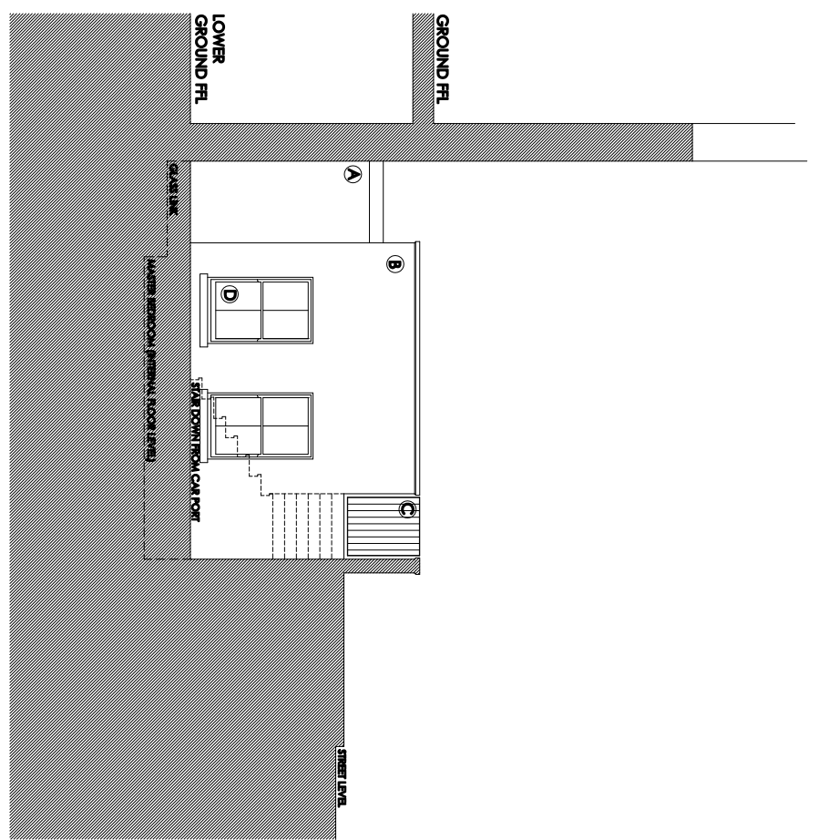
PROPOSED SIDE ELEVATION - LOWER GROUND FRONT COURTYARD 1:100@A3
