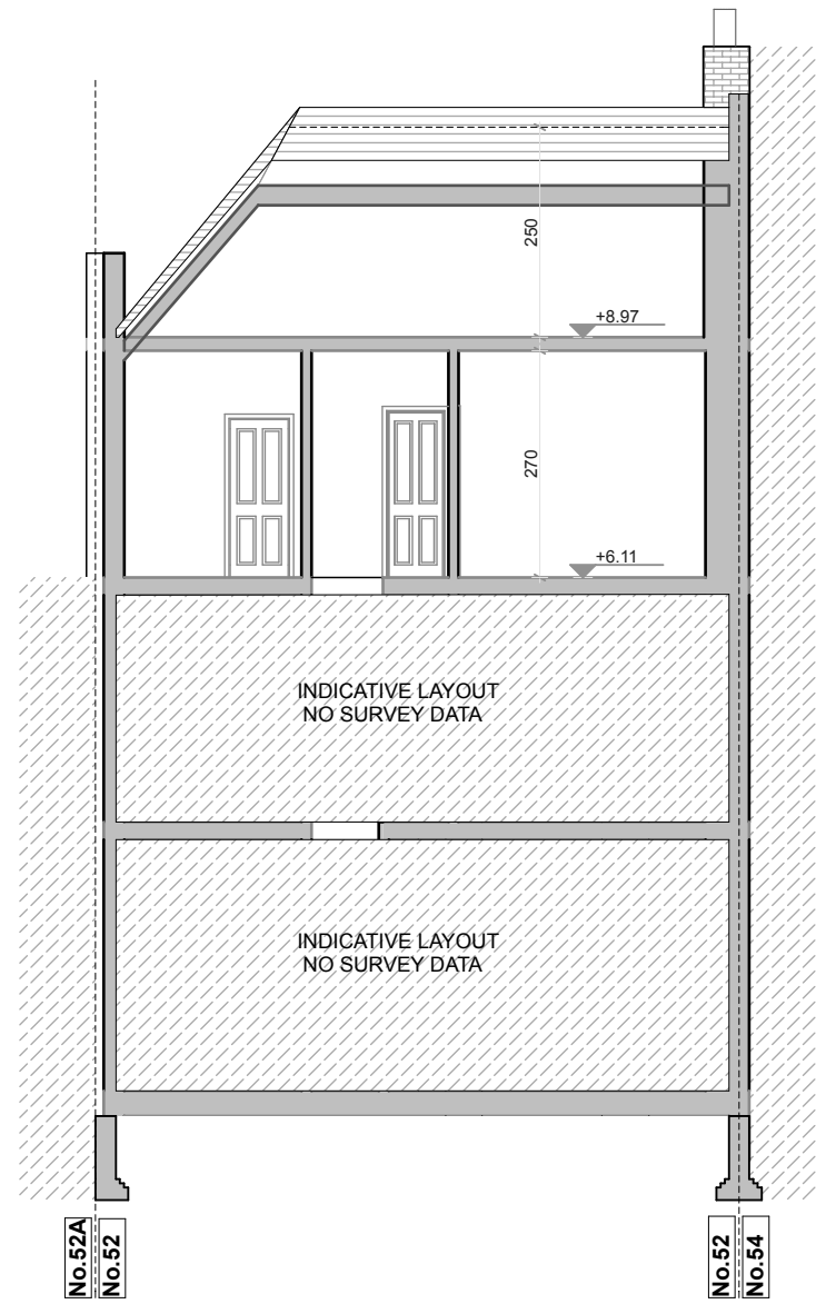
SECTION B-B EXISTING 1:100
