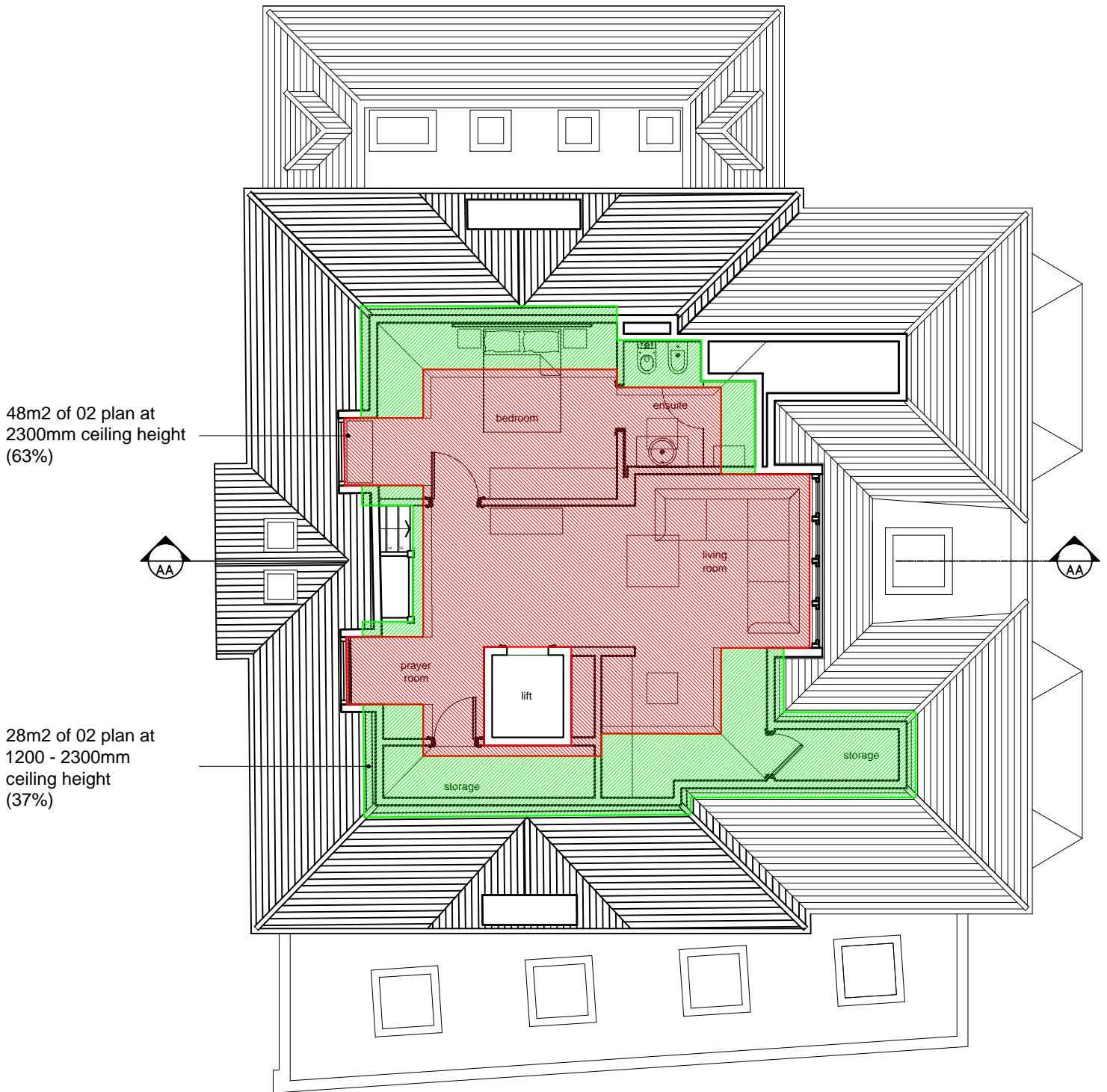
36 Heath Drive 02 floor plan showing ceiling height percentages (not to scale)
