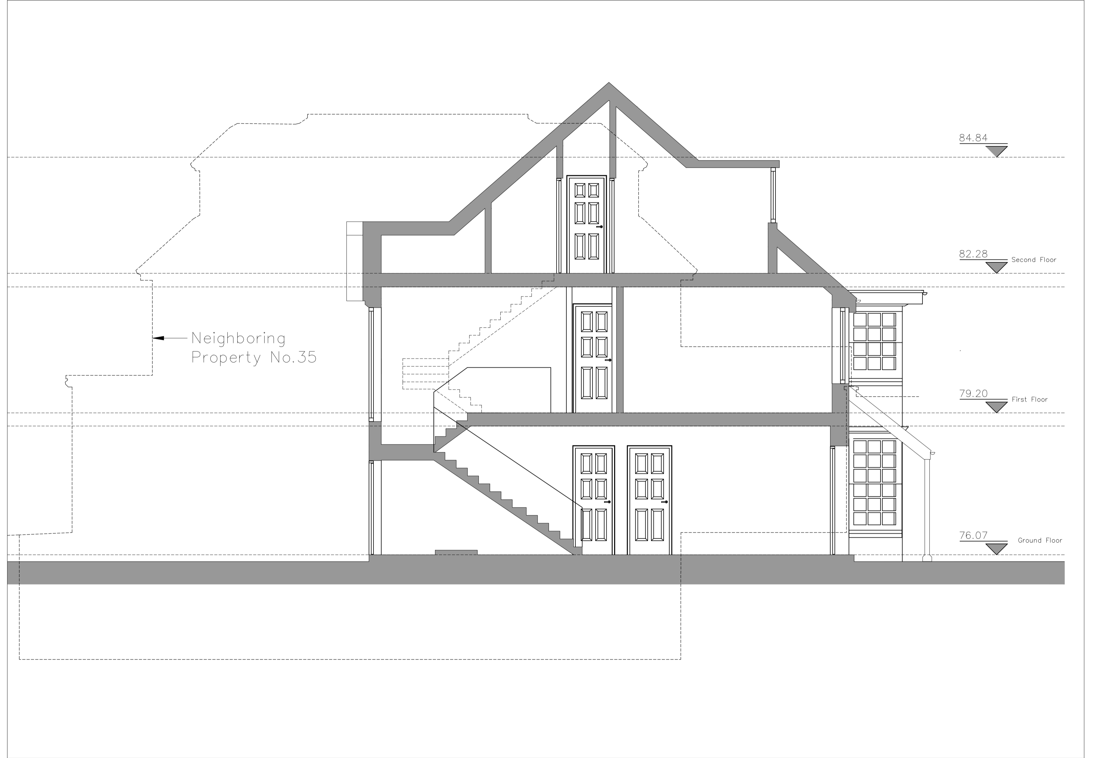
Existing section AA
