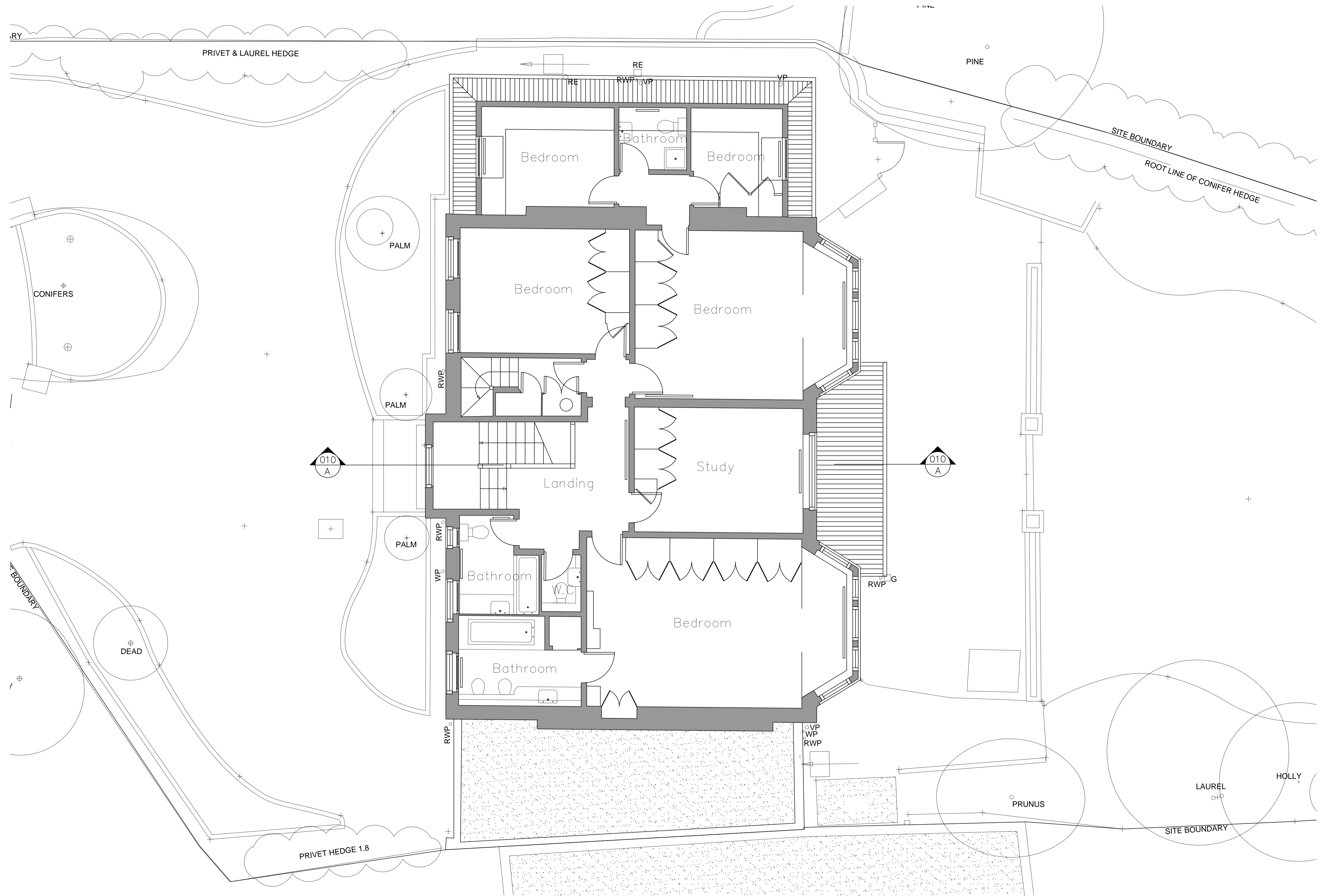
Existing first floor plan
