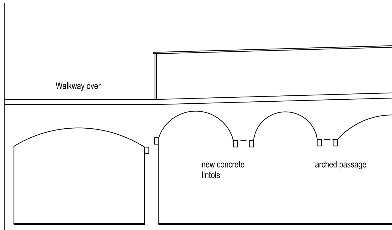
Section B B through brick arch passage
