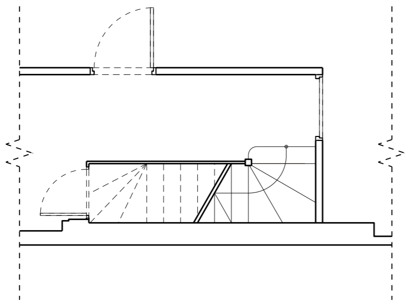
01 Existing Third Floor Plan 1:50
