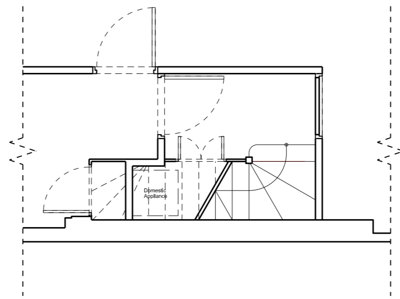
02 Proposed Third Floor Plan 1:50
