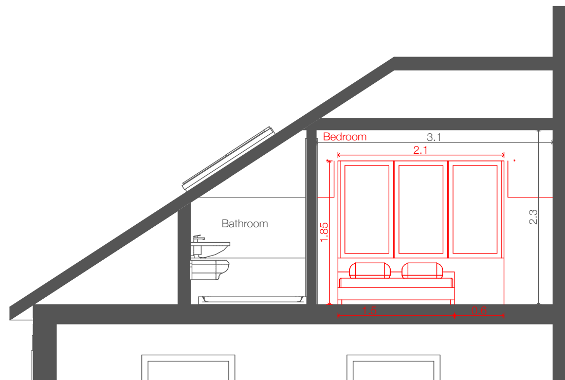
Section B
