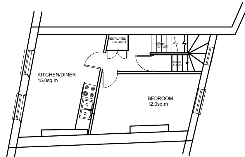
EXISTING SECOND FLOOR PLAN - FLAT B
