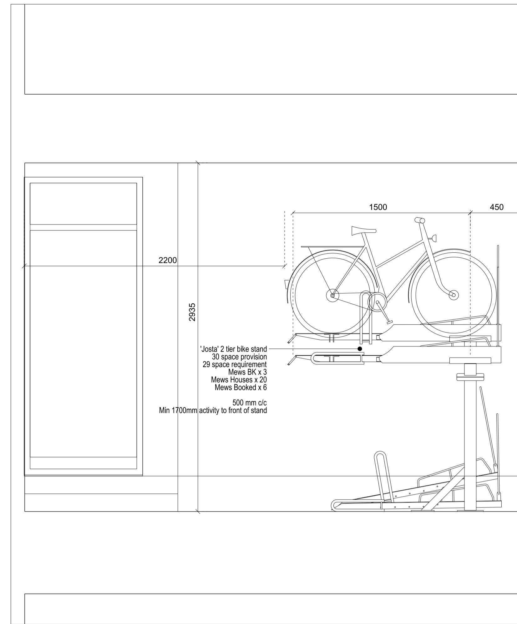
02048902 NO. 12 Section of Blemundsbury Houses cycle store
