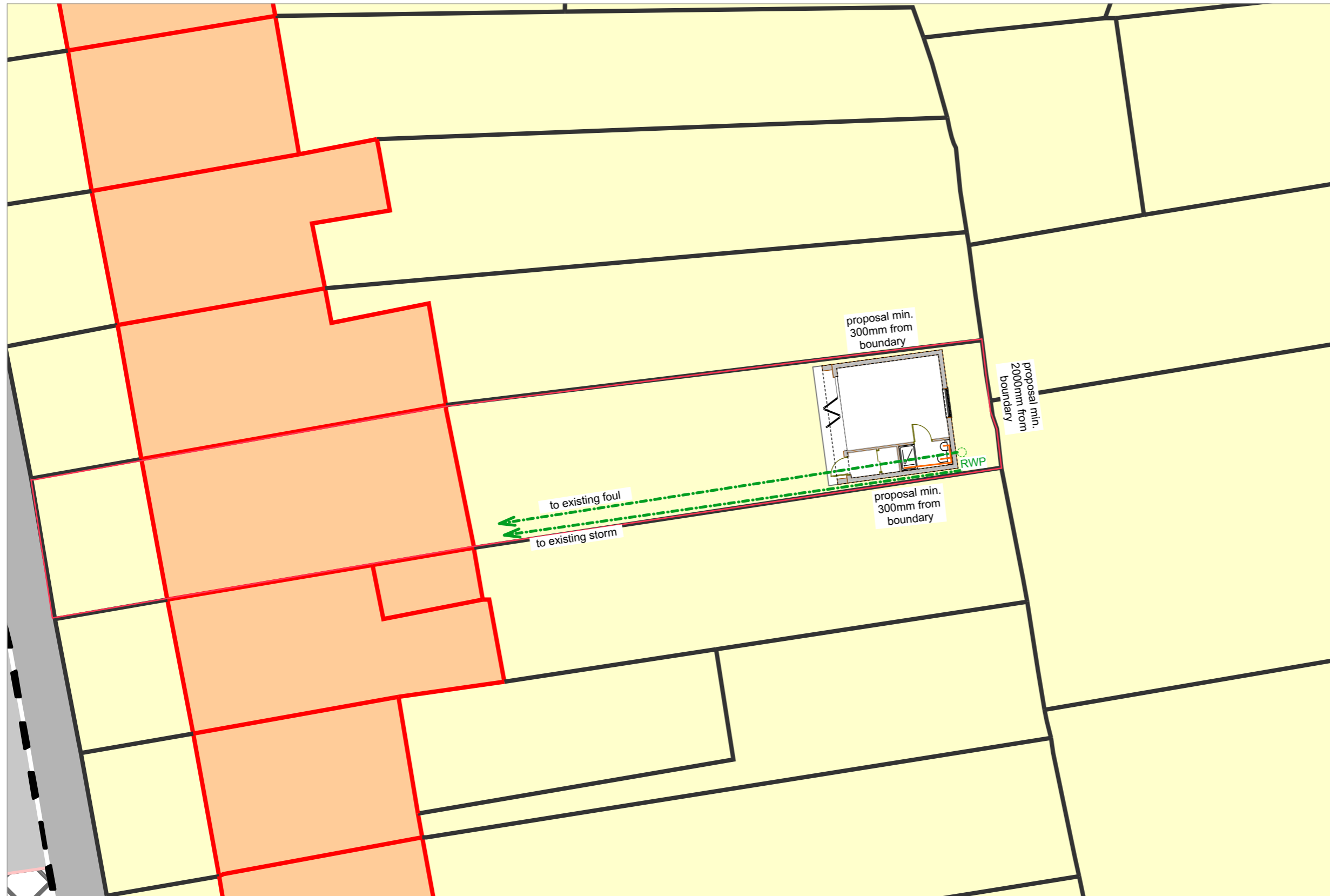
Site Plan- 1:200 (at A3)
