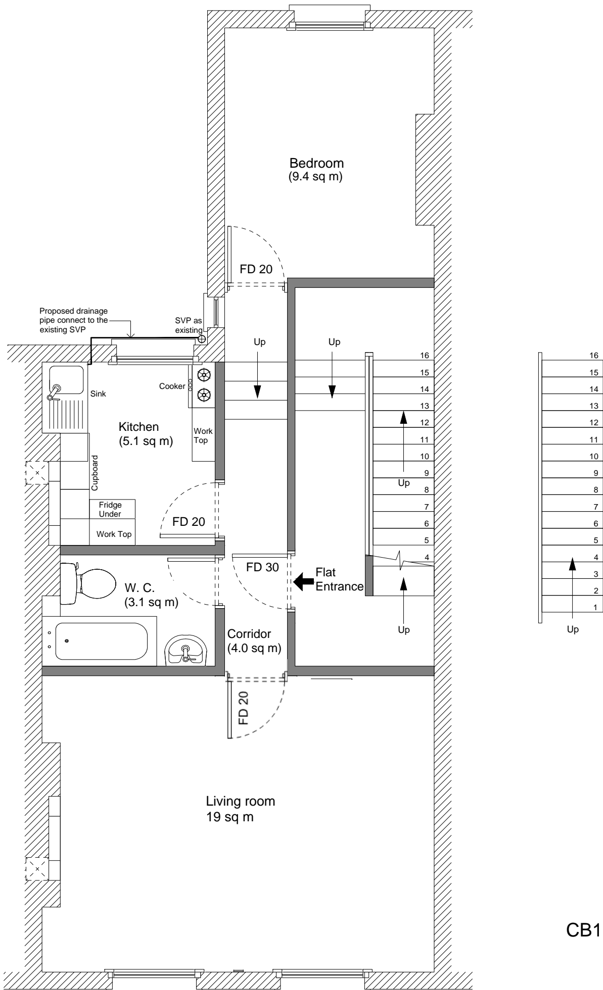
FIRST FLOOR PLAN AS PROPOSED SCALE: 1:50
