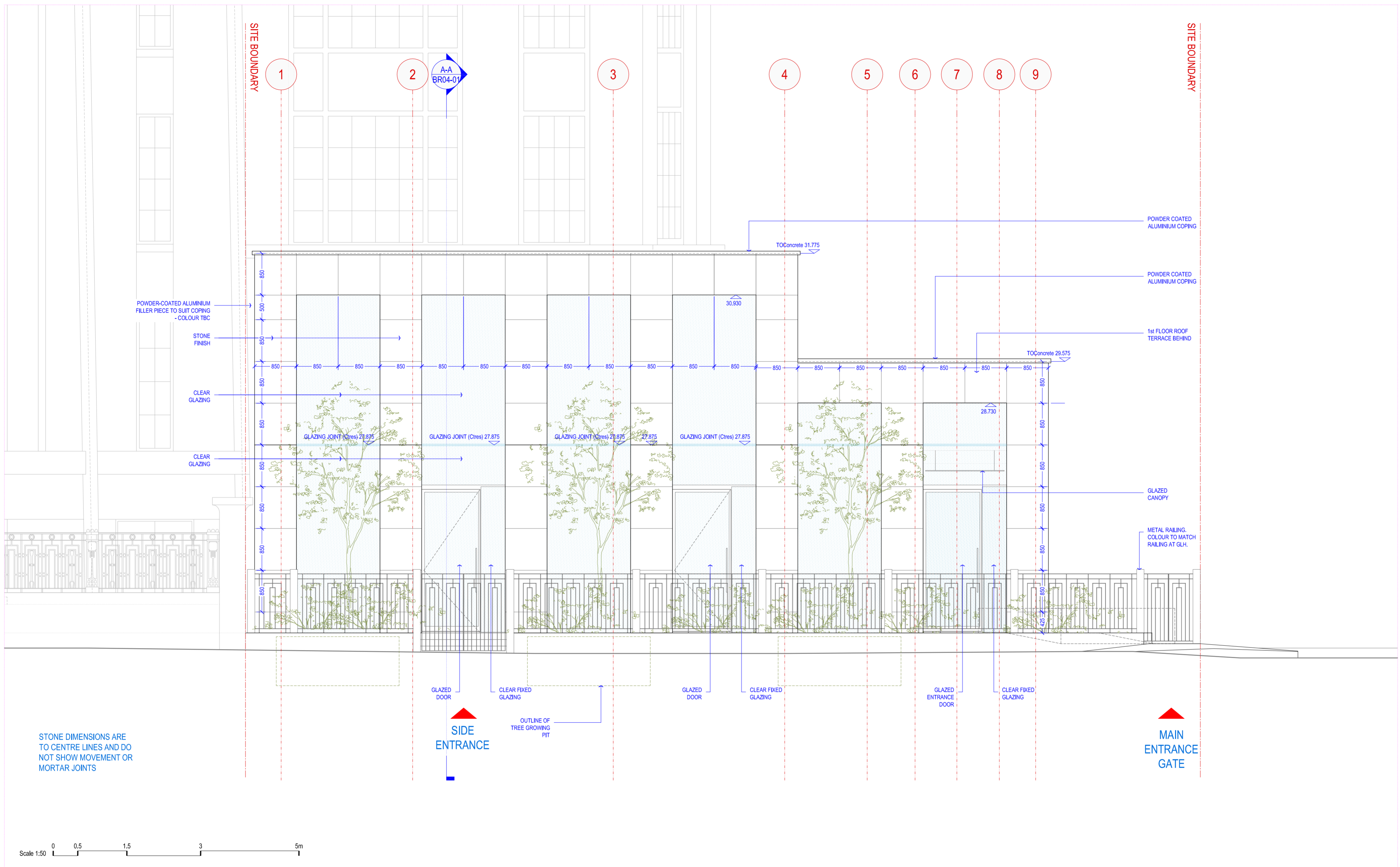
[01] Elevation A - Front Elevation, Hampstead Road (East)
