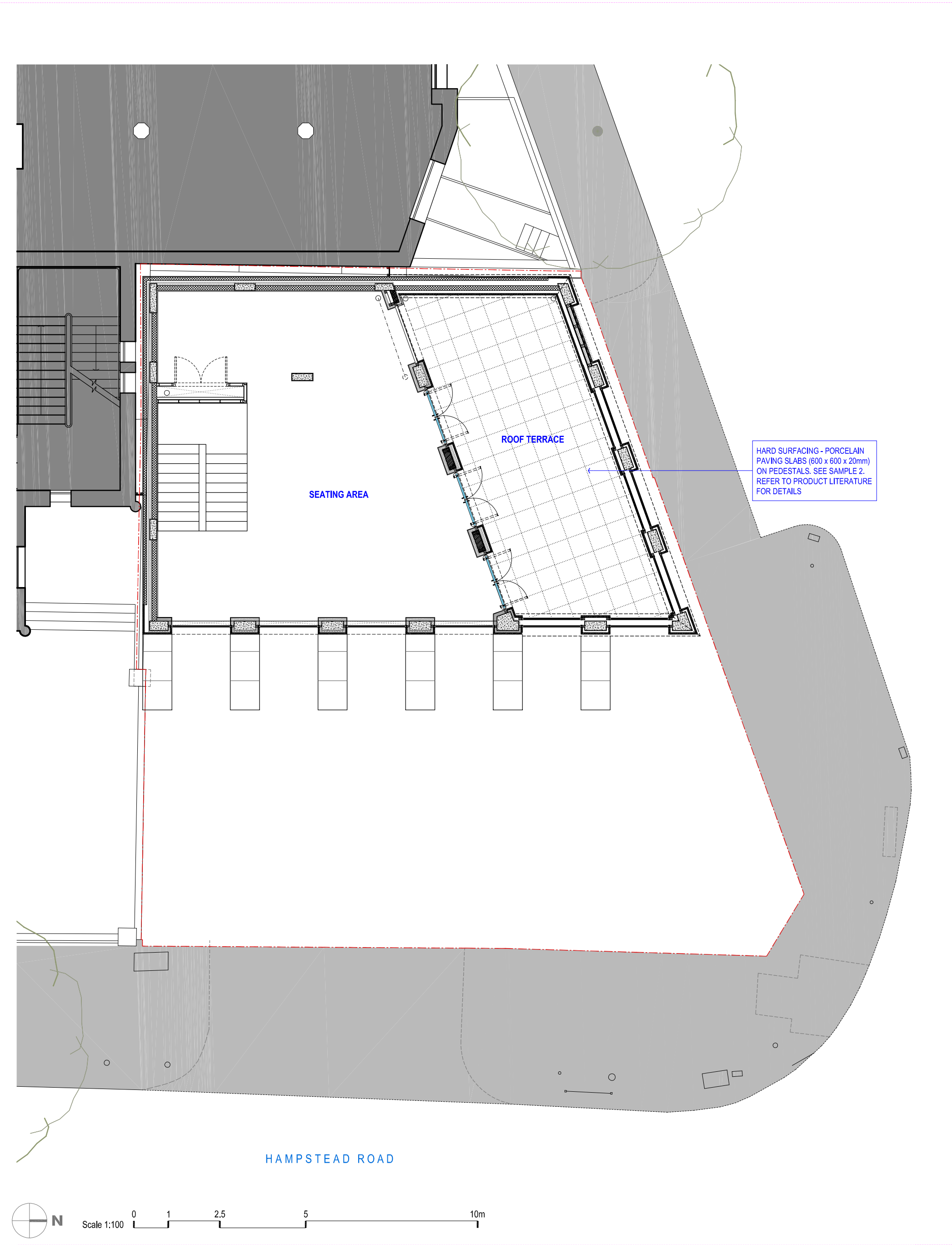
[01] PROPOSED 1ST FLOOR LANDSCAPE PLAN - 1:100
