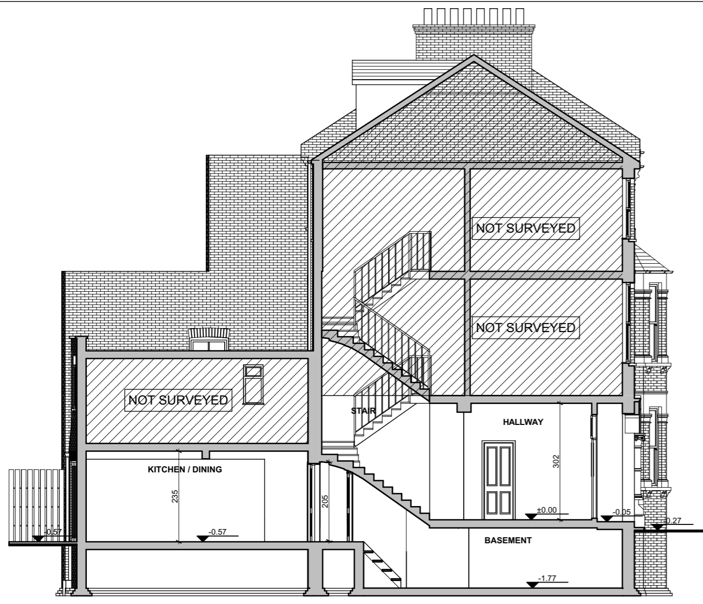
SECTION AA - PROPOSED
