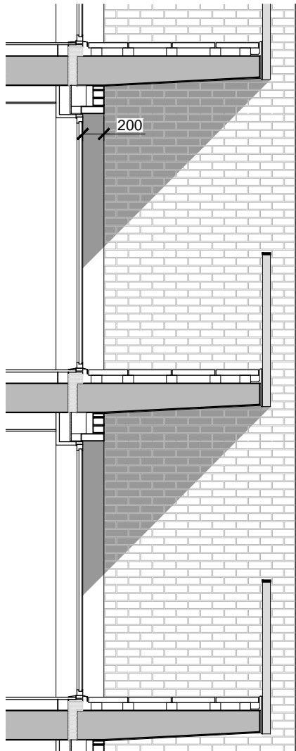
SECTION DETAIL 01b (in limited locations where tapered balcony slab required)
