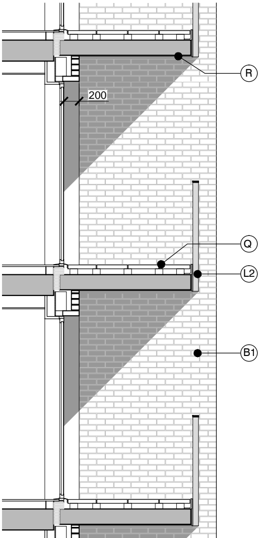
SECTION DETAIL 01a
