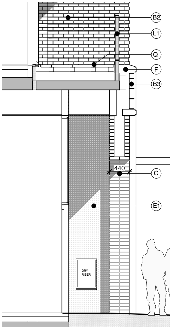
SECTION DETAIL 01
