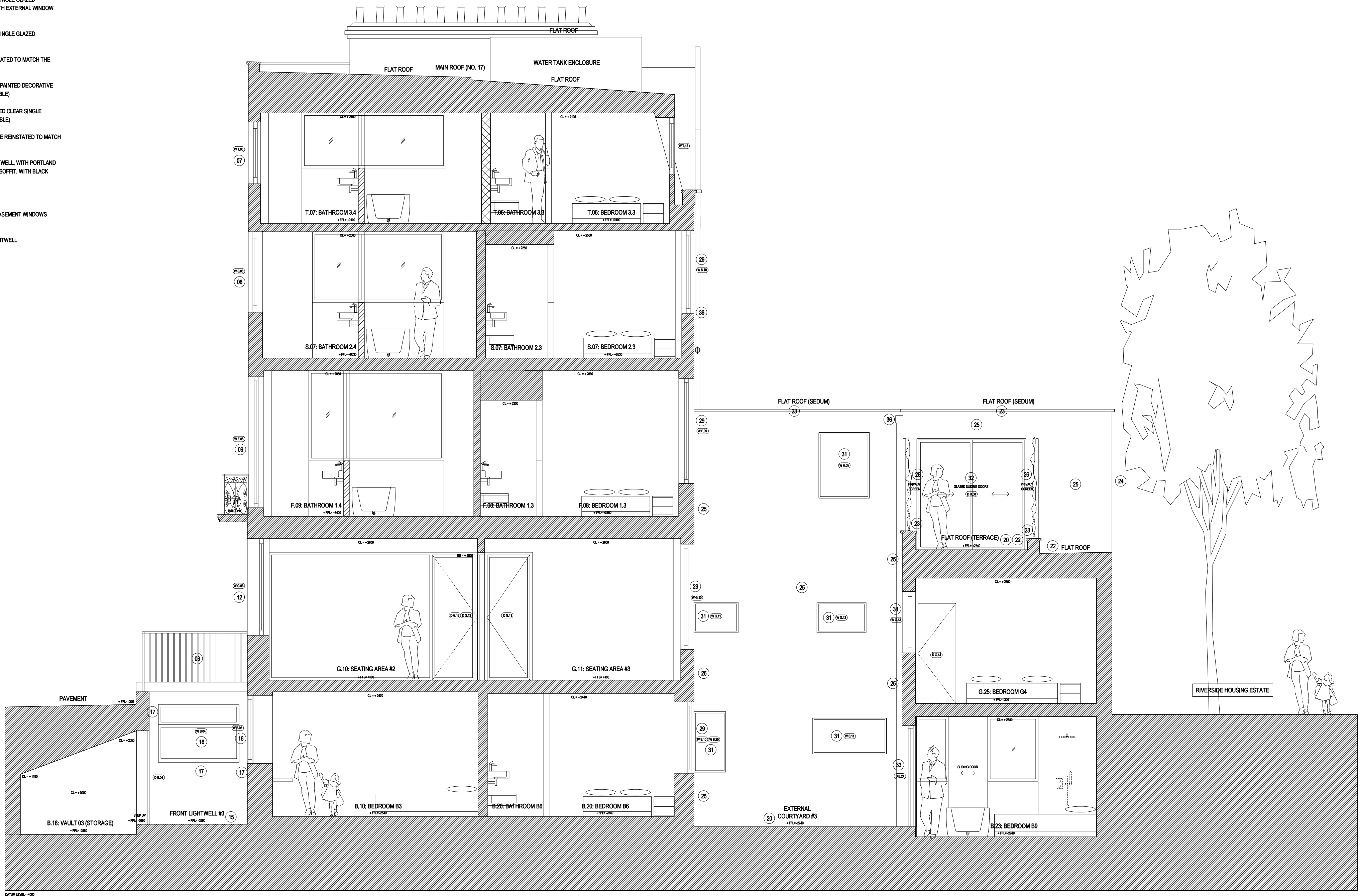
10 PROPOSED SECTION 10 (15-12-10) Scale 1:50 (@A1 SIZE)
