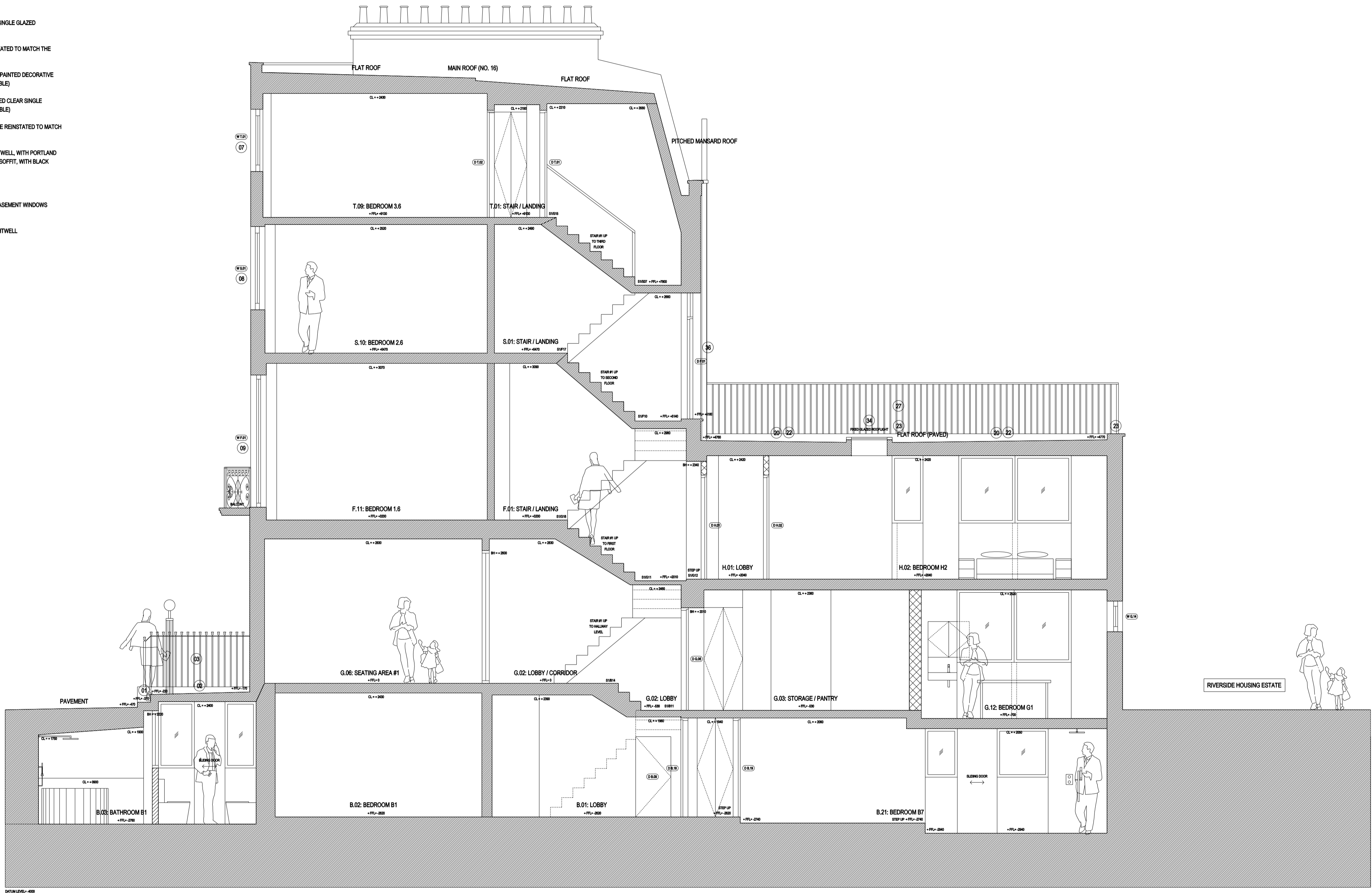
05 PROPOSED SECTION 05 (15-12-05) Scale 1:50 (@A1 SIZE)
