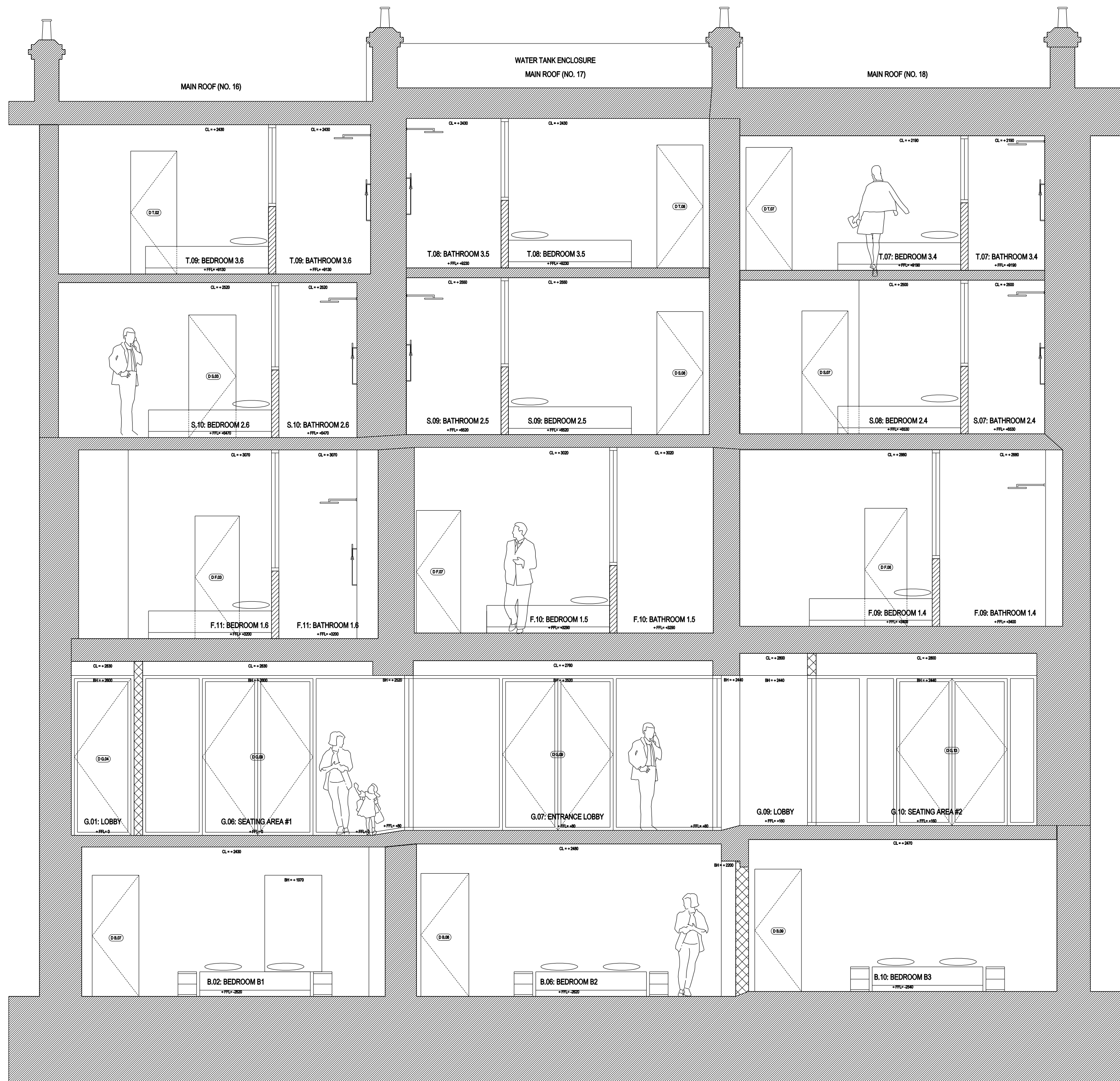
02 PROPOSED SECTION 02 (15-12-02) Scale 1:50 (@A1 SIZE)
