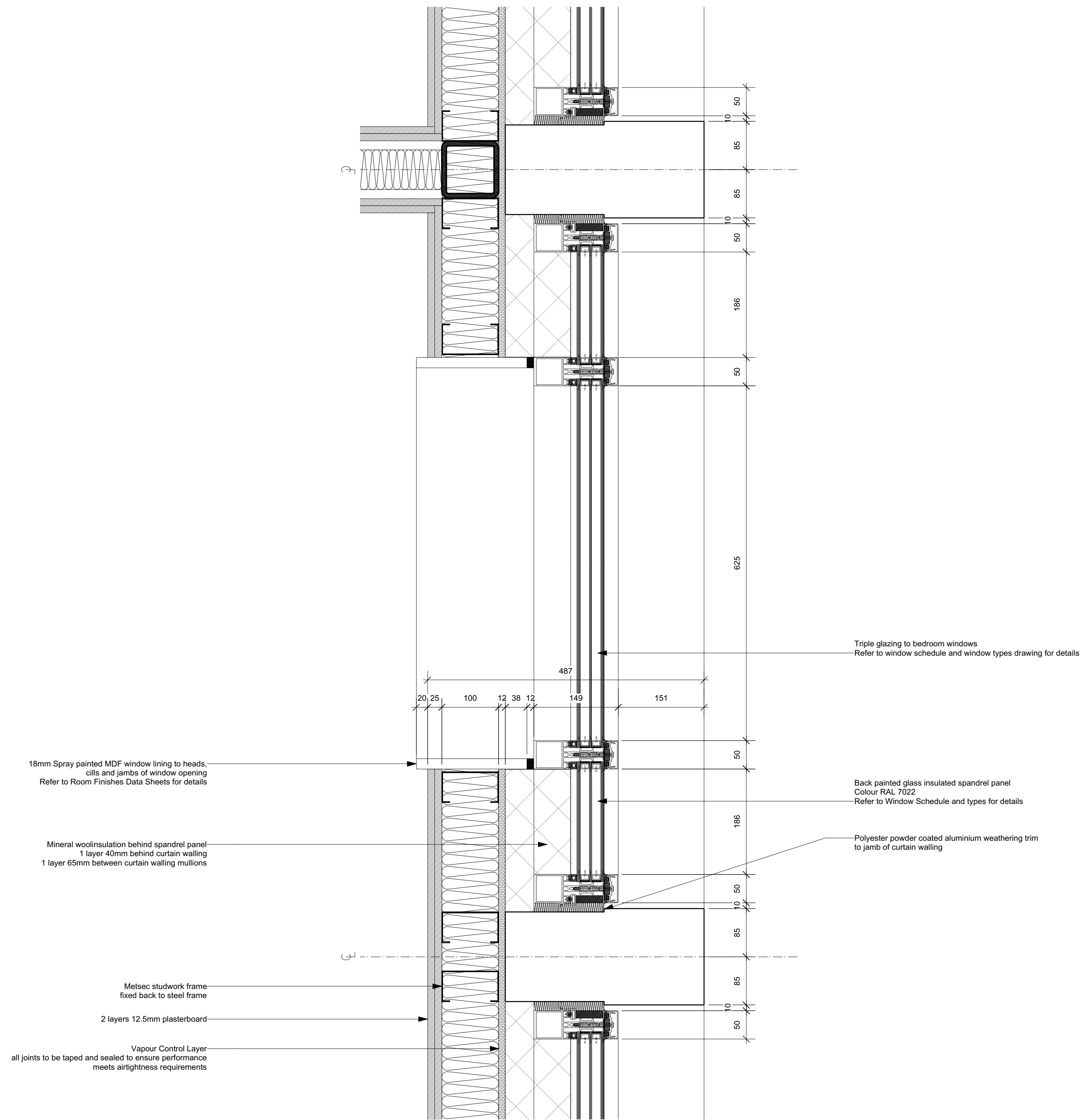
6TH FLOOR EXTERNAL WINDOW JAMB DETAIL NORTH ELEVATION
