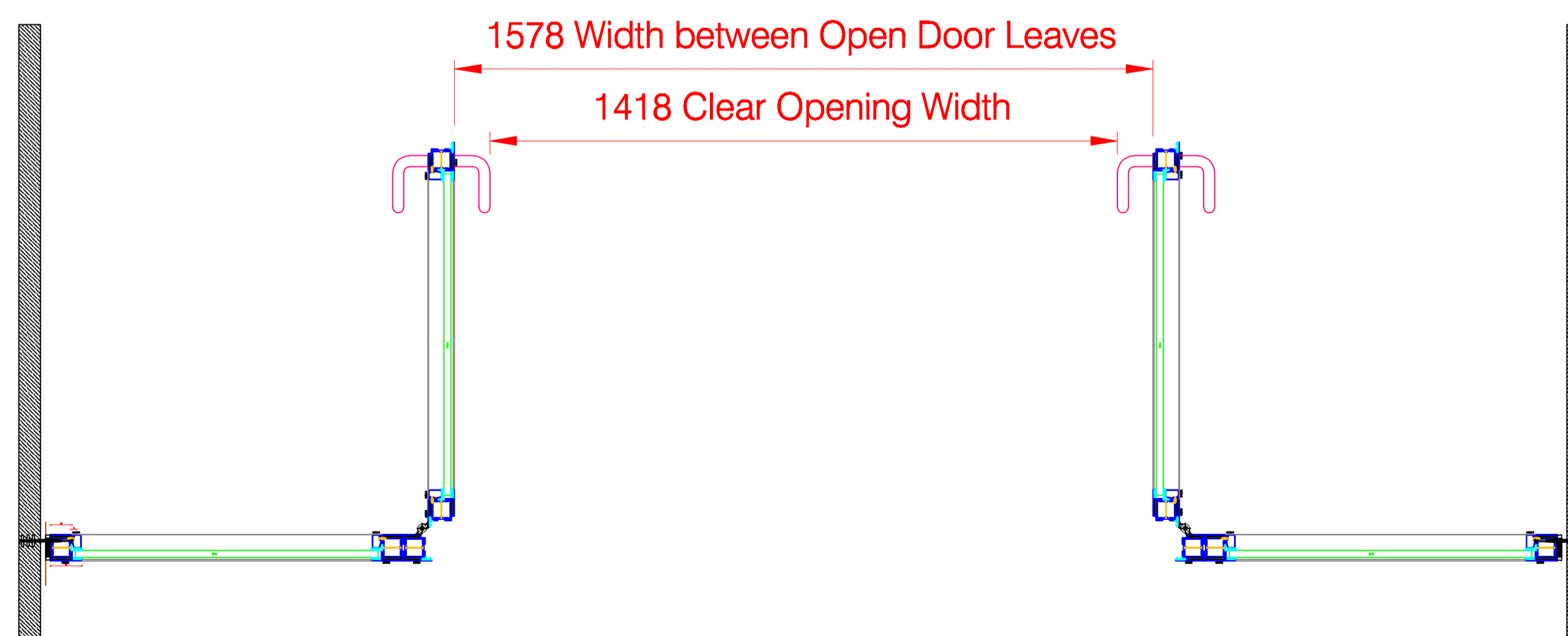
PLAN SHOWING DOORS IN OPEN POSITION Scale 1:10 @ A1
