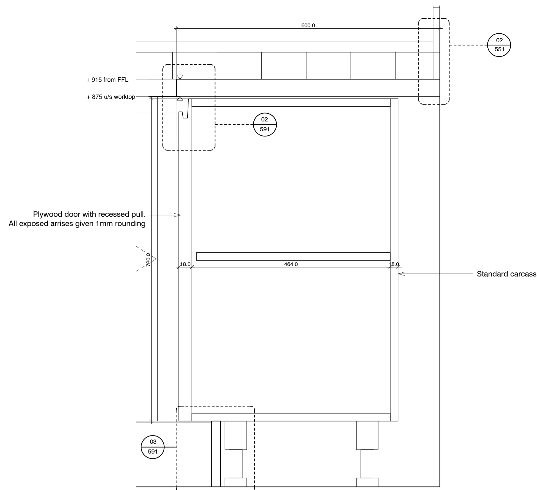
01 Cross section 579
