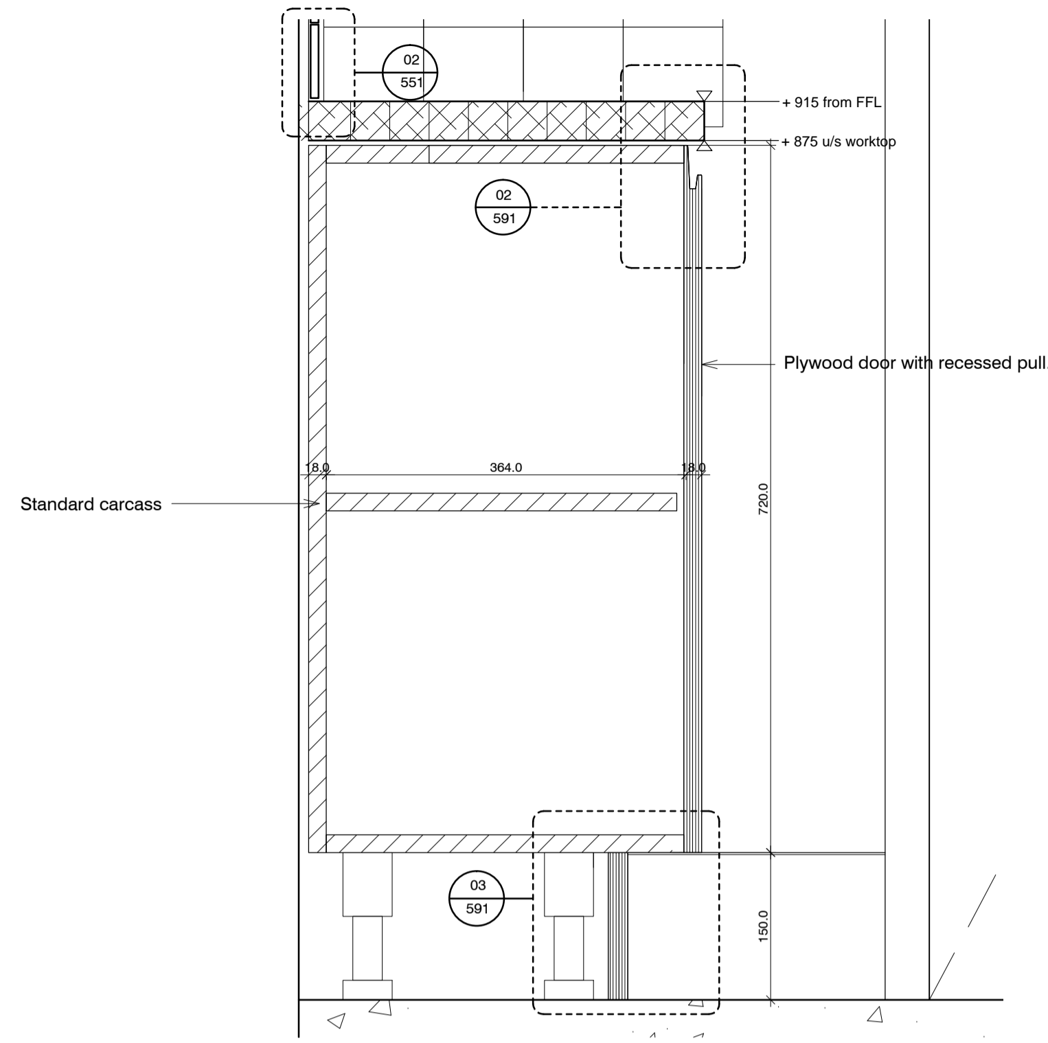
01 Cross section 572
