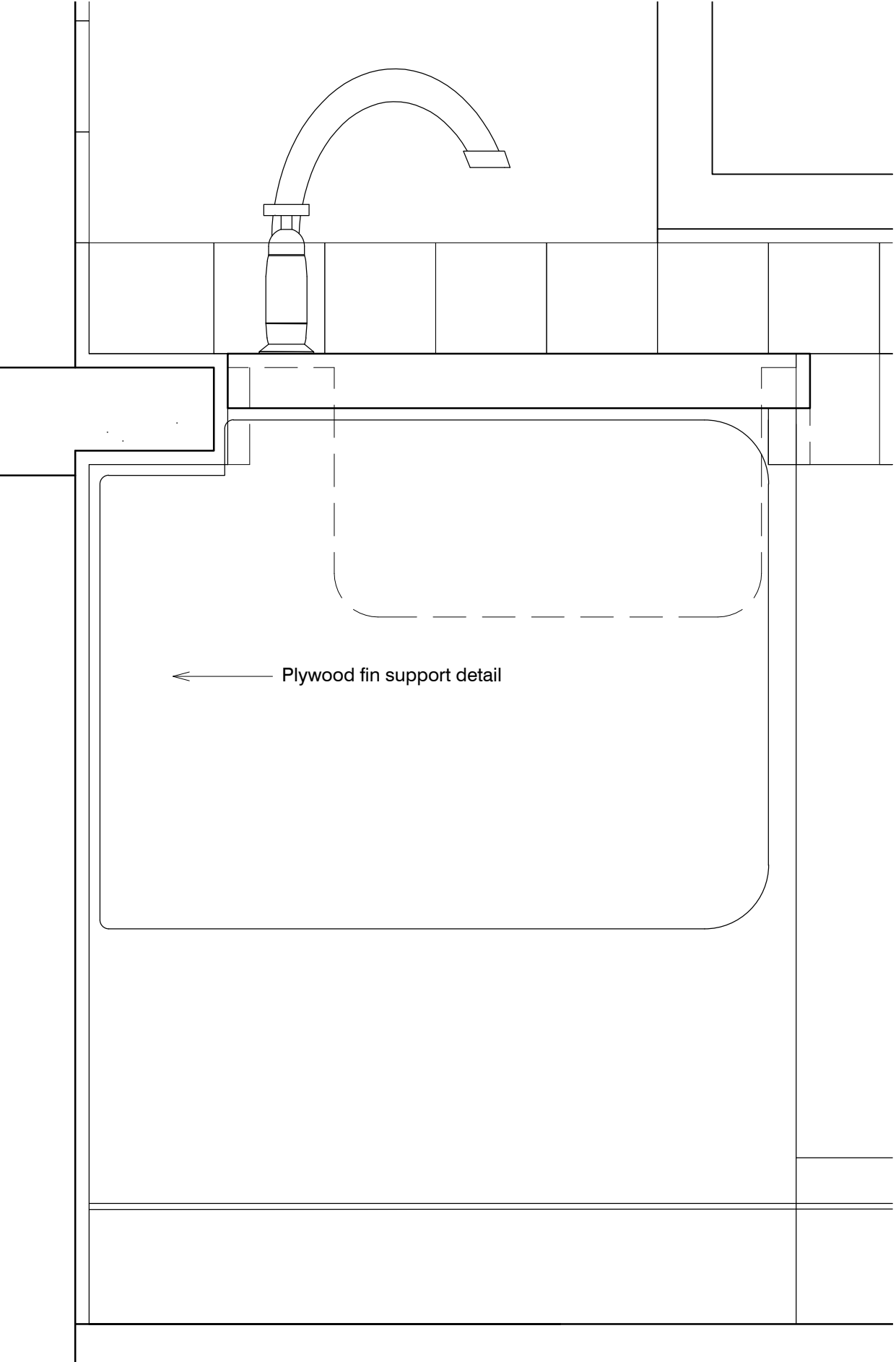
01 Cross section 530
