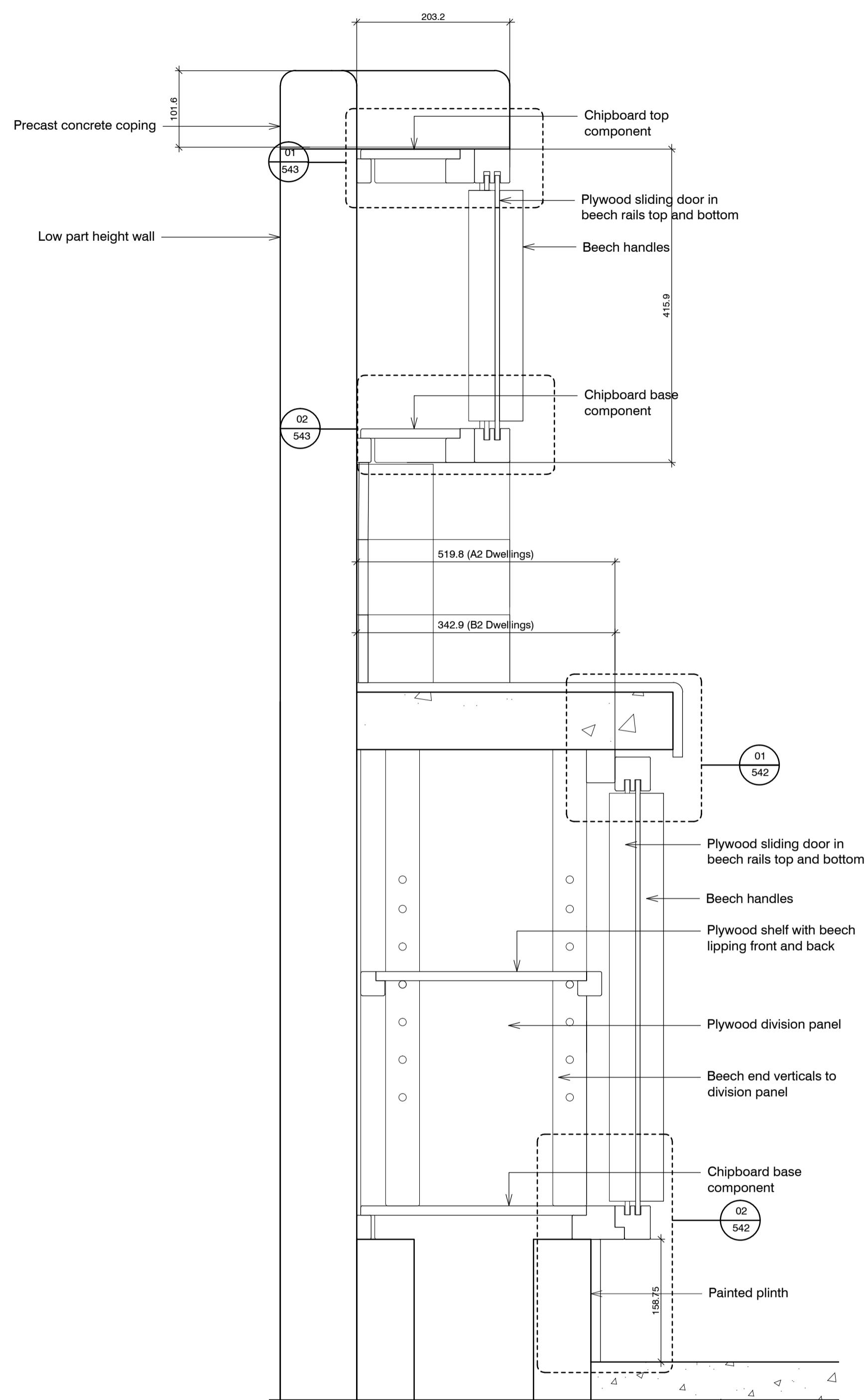
01 Cross section 524
