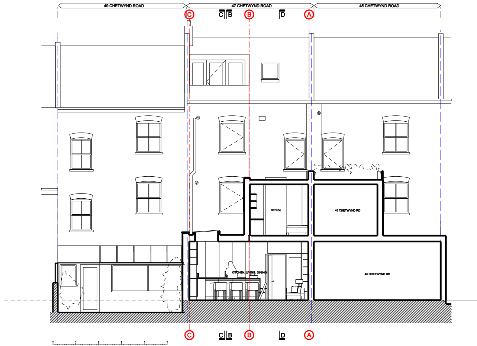
01 SECTION AA PROPOSED SCALE 1:100 AT A3
