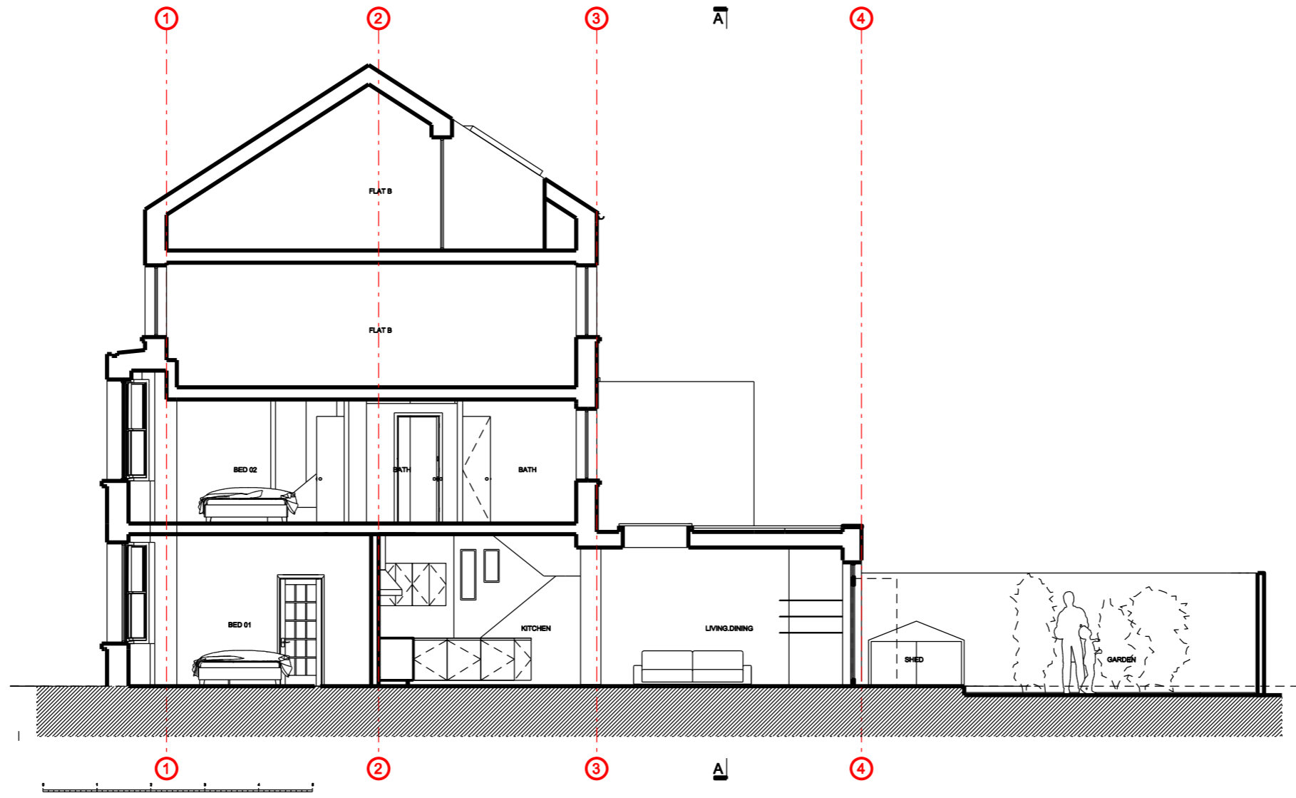
01 SECTION BB EXISTING SCALE 1:100 AT A3
