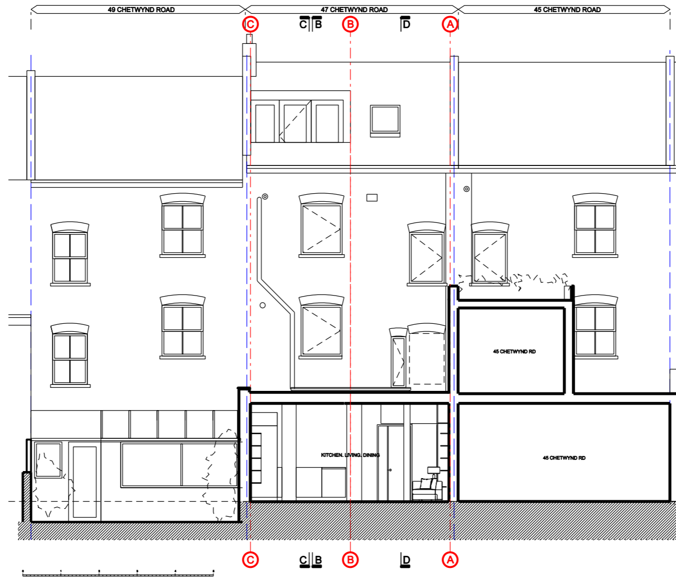
01 SECTION AA EXISTING SCALE 1:100 AT A3
