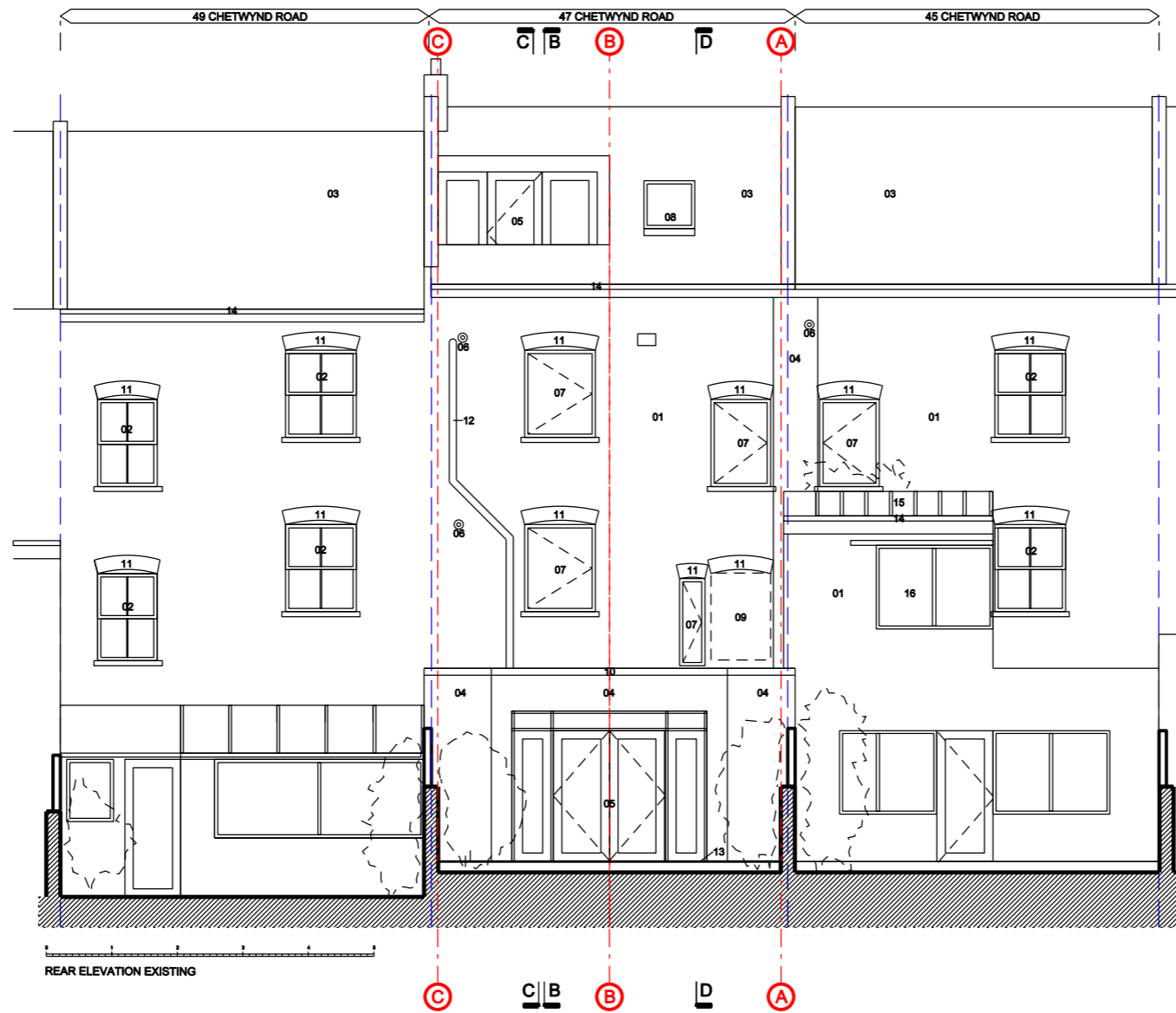
01 ELEVATION EXISTING SCALE 1:100 AT A3
