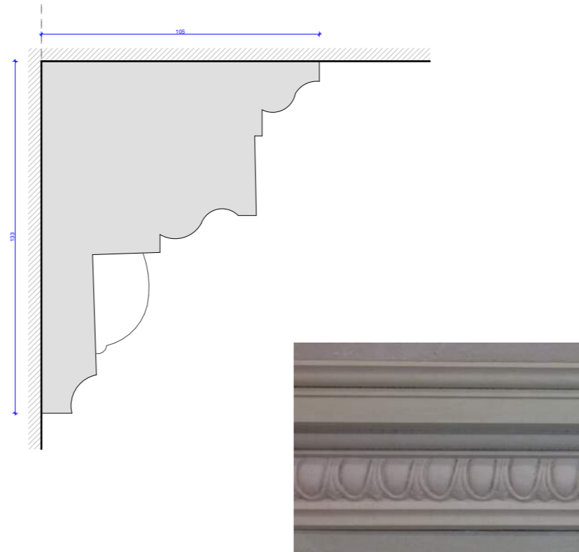
1:2 New cornice London Plaster Craft : CR 193
