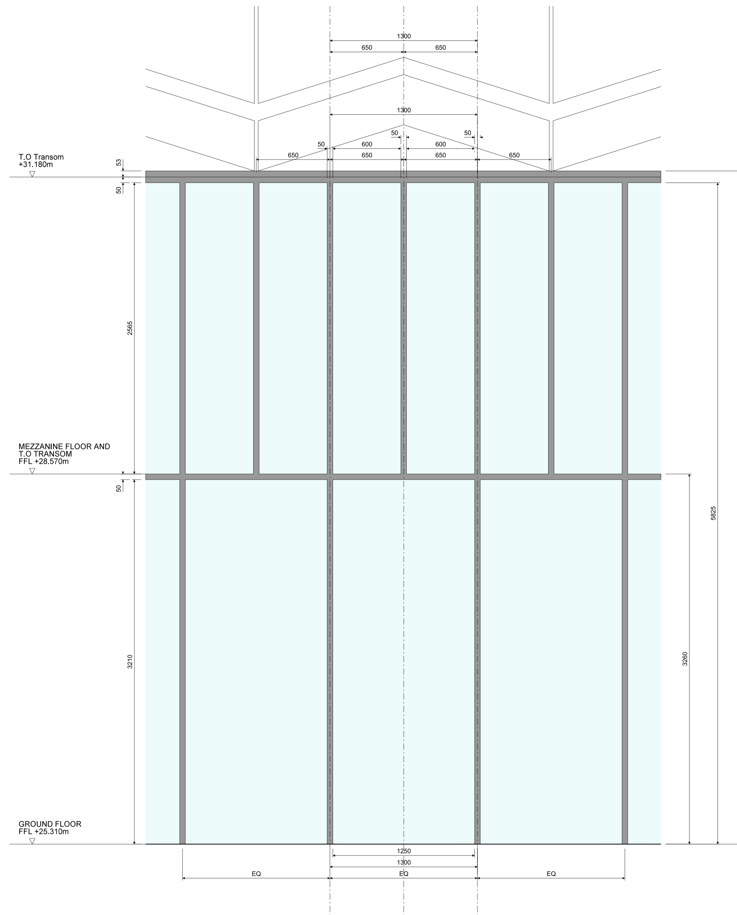
1 ELEVATION 1:20
