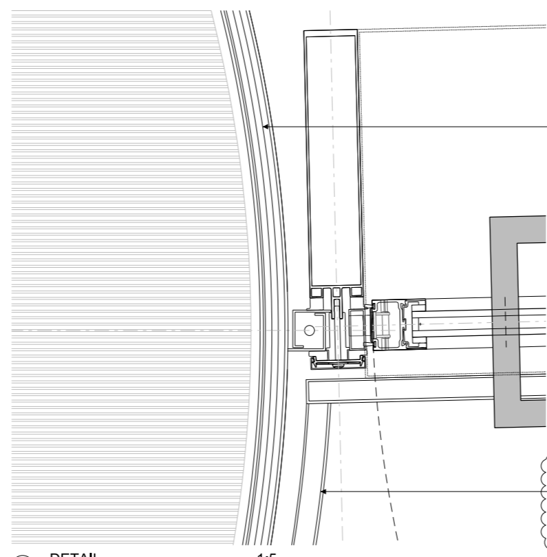
2 DETAIL 1:5
