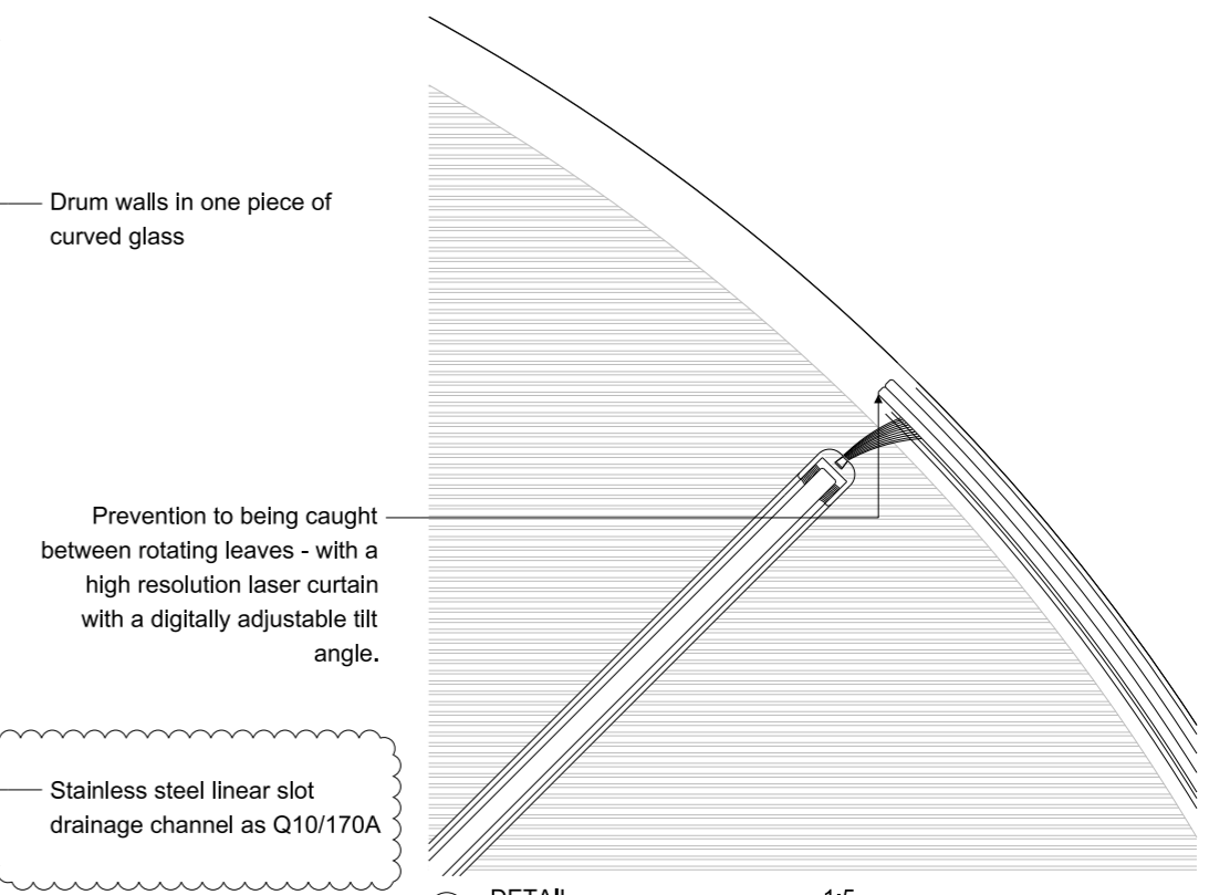
4 DETAIL 1:5
