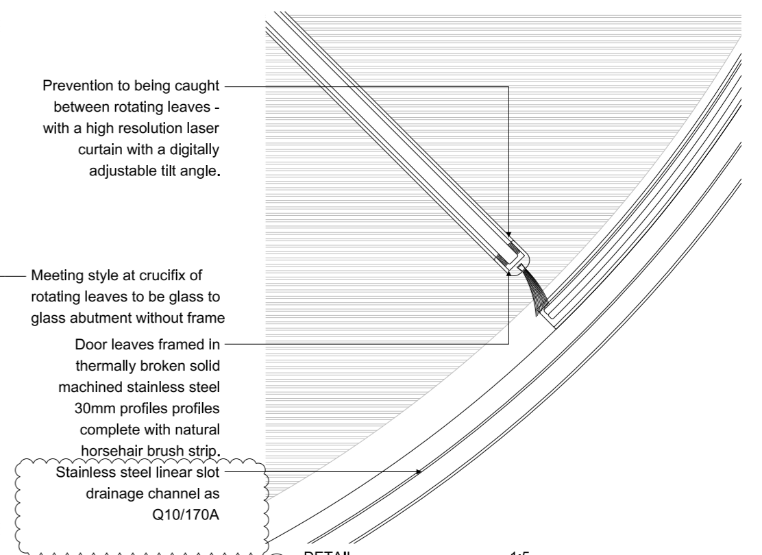
5 DETAIL 1:5
