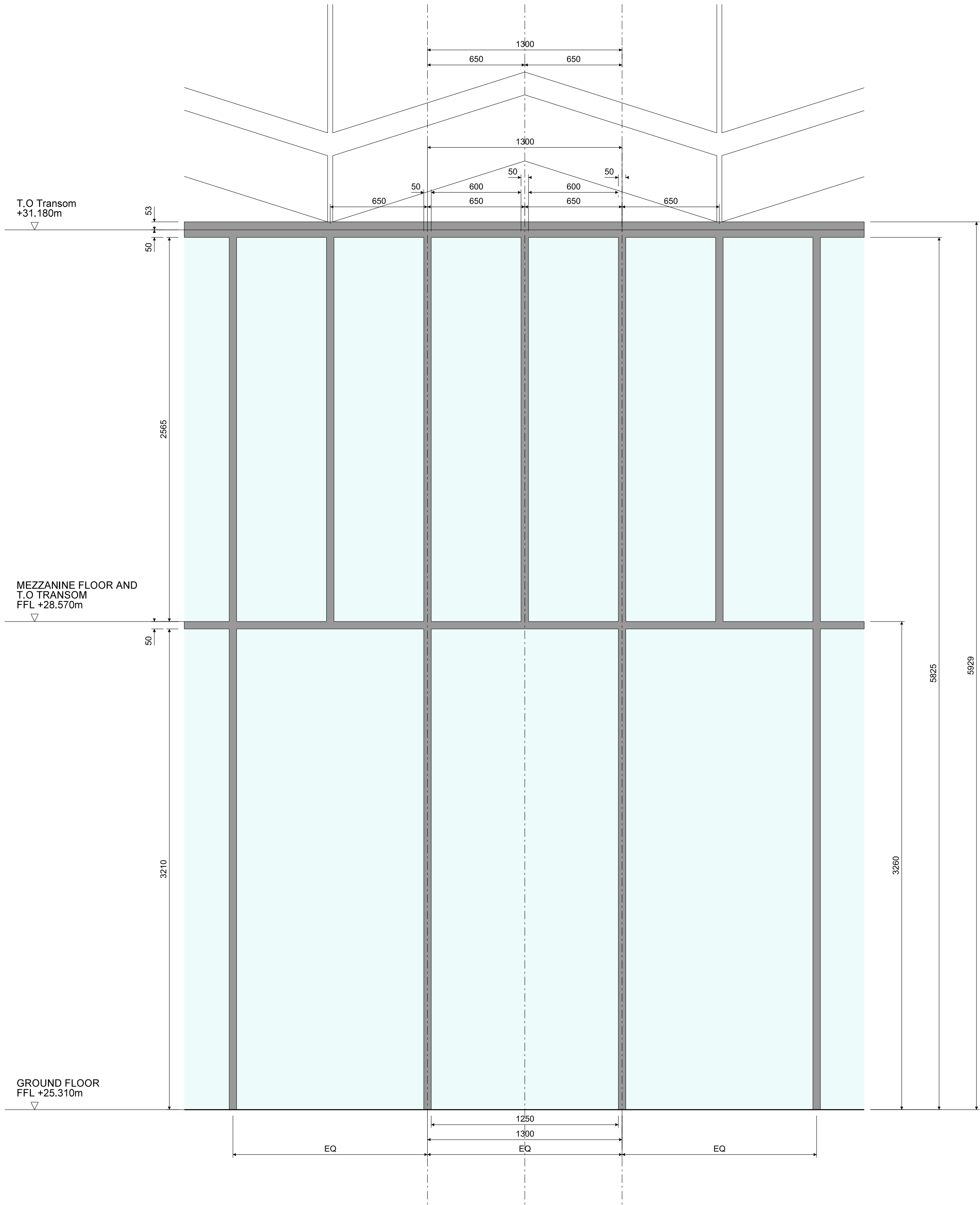
1 ELEVATION 1:20
