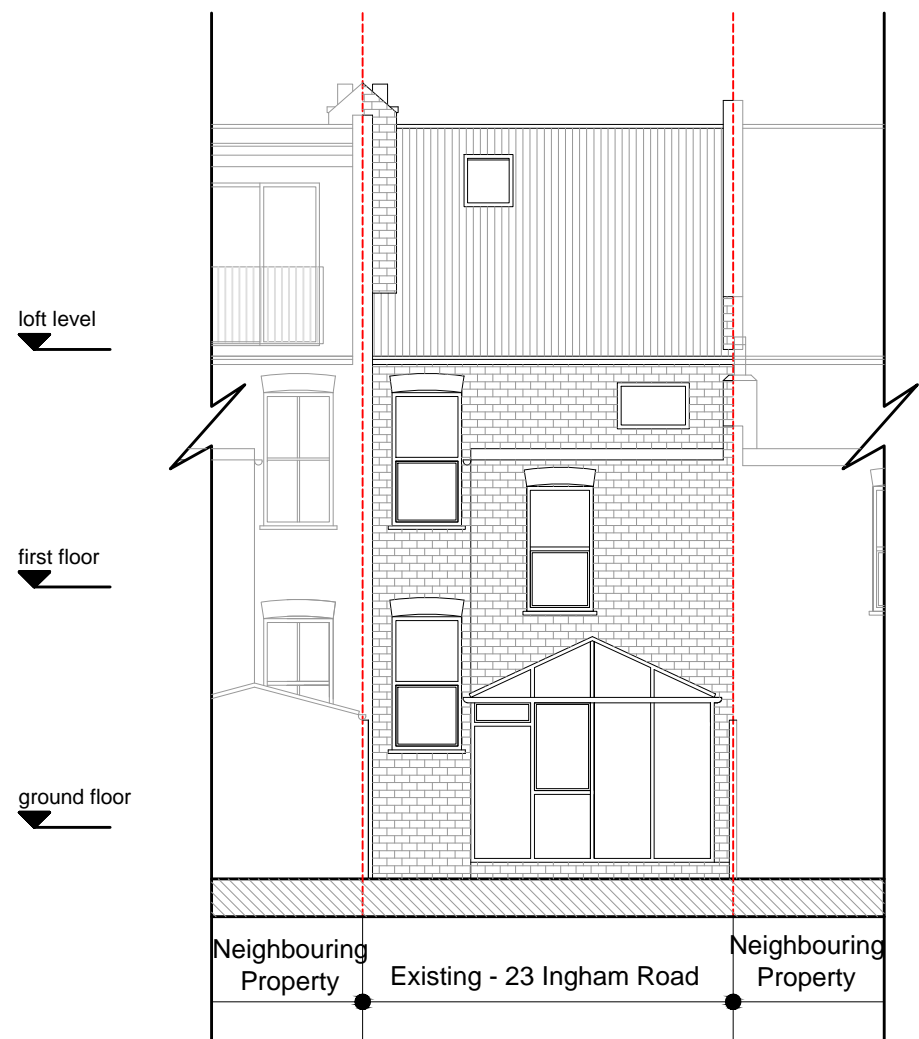
REAR ELEVATION
