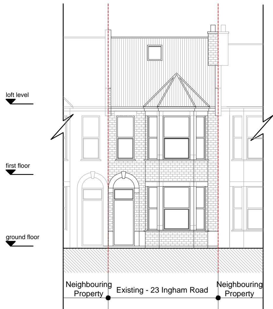
FRONT ELEVATION
