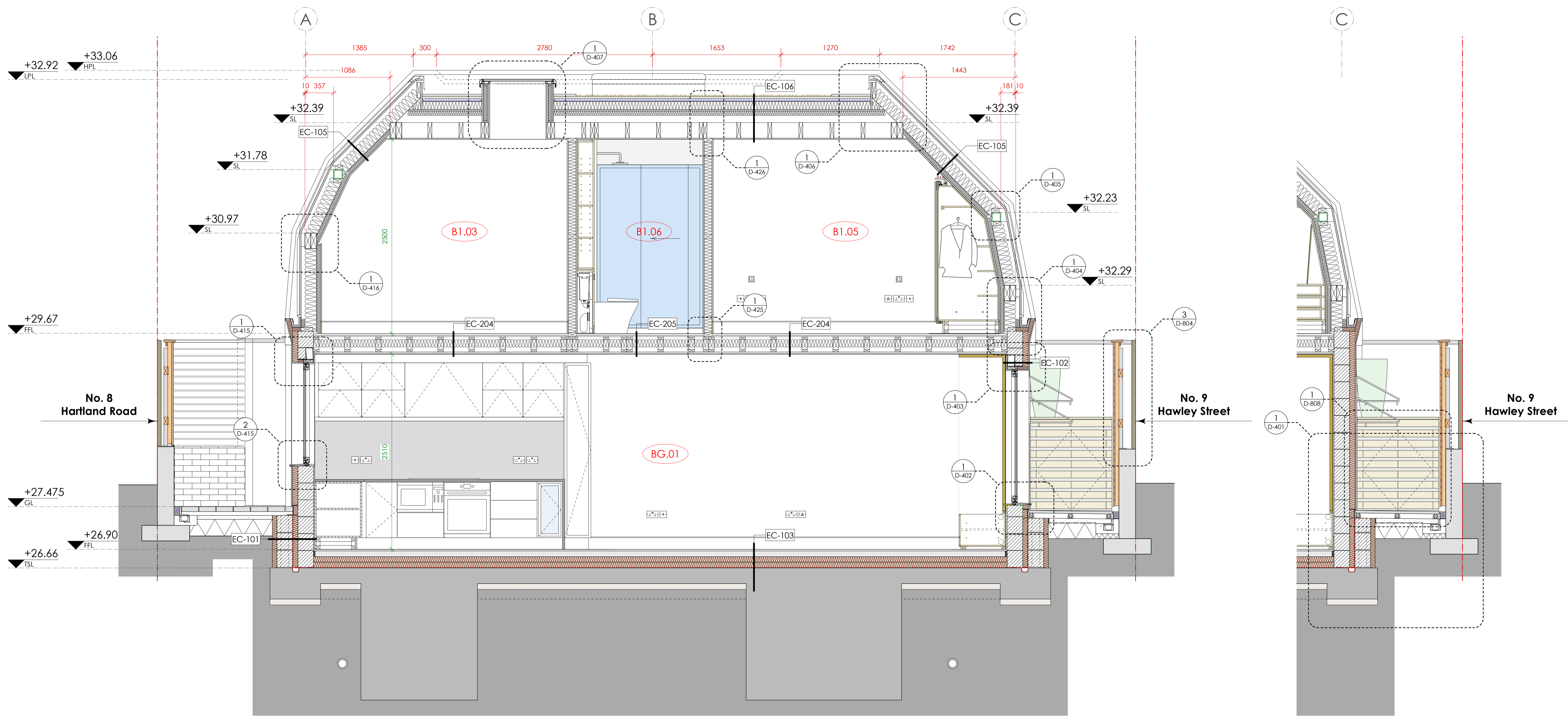
1 Proposed Detailed Cross Section D-303 scale 1:25 @ A1 / 1:50 @ A3
