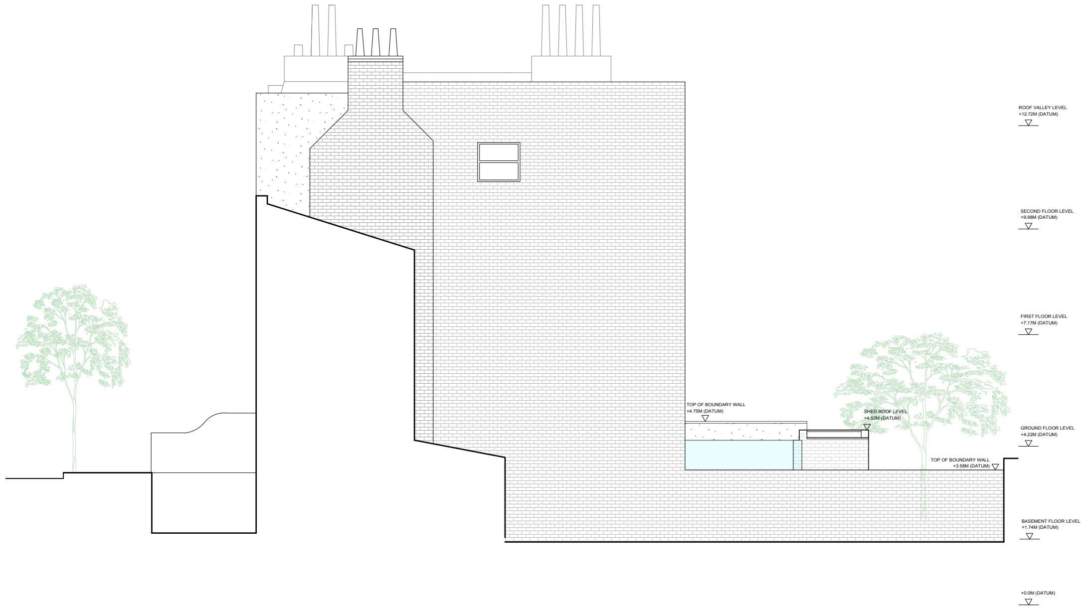
1 EXISTING WEST ELEVATION SCALE 1:100@A3
