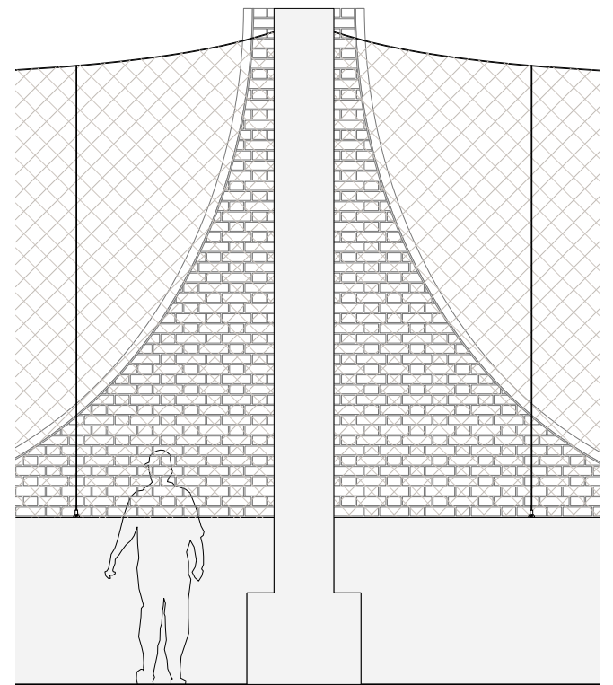
Pitch-Side Elevation 1:25
