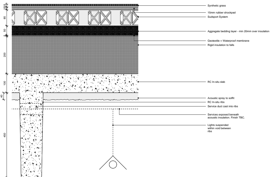
D01 MUGA Floor Build-Up 1:5
