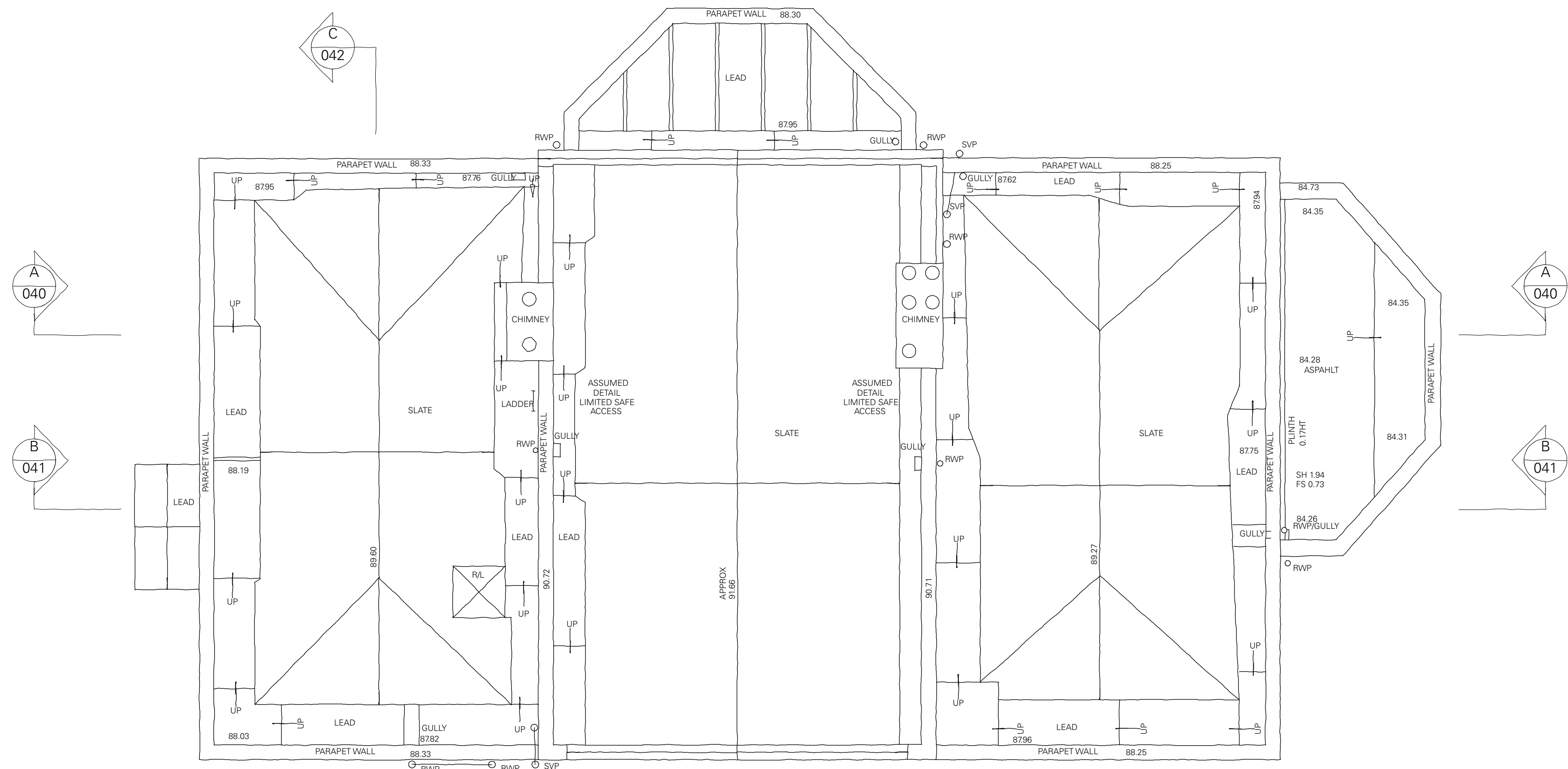
B PLAN: EXISTING ROOF 1.50 @ A1, 1.100 @ A3
