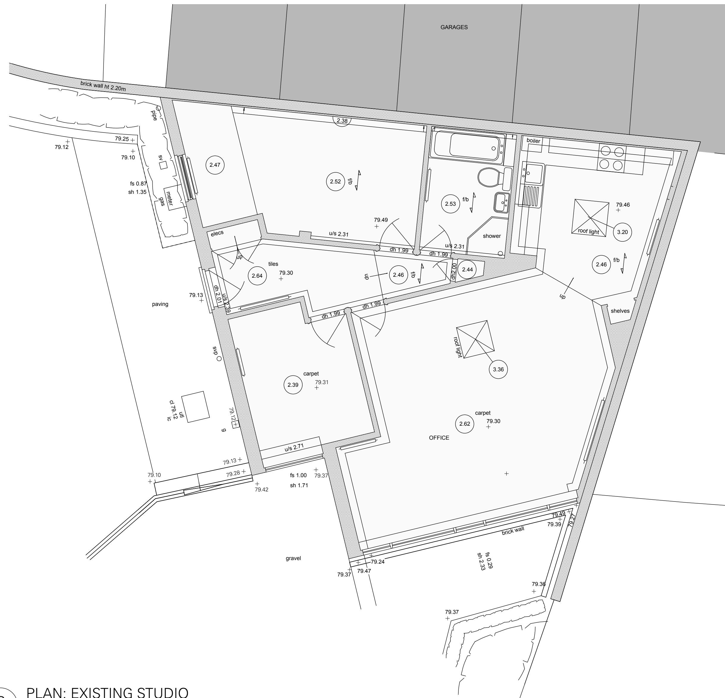
C PLAN: EXISTING STUDIO 1.50 @ A1, 1.100 @ A3
