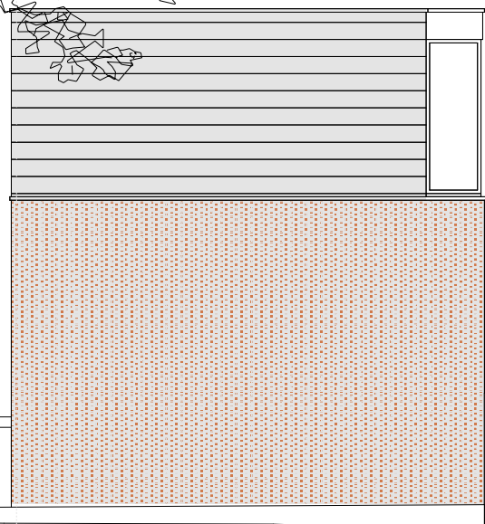
North Elevation 66 Fitzjohns Avenue
