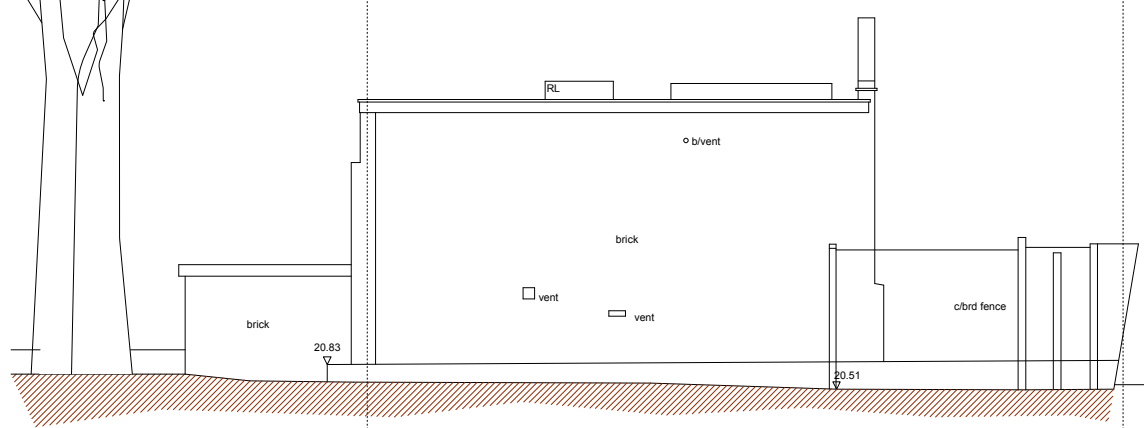
South Elevation 66 Fitzjohns Avenue
