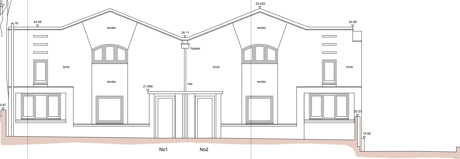
Front West Elevation 66 Fitzjohns Avenue
