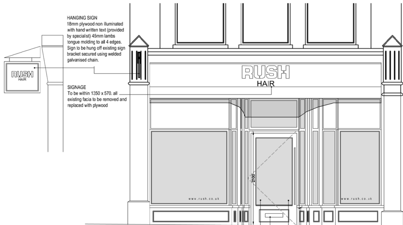
Proposed Shop Front: 1:50 Scale
