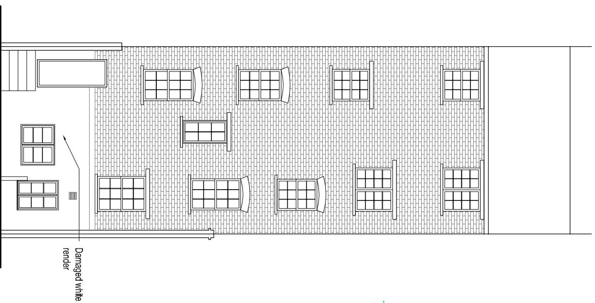
REAR ELEVATION PRIOR TO THE REAR EXTENSION
