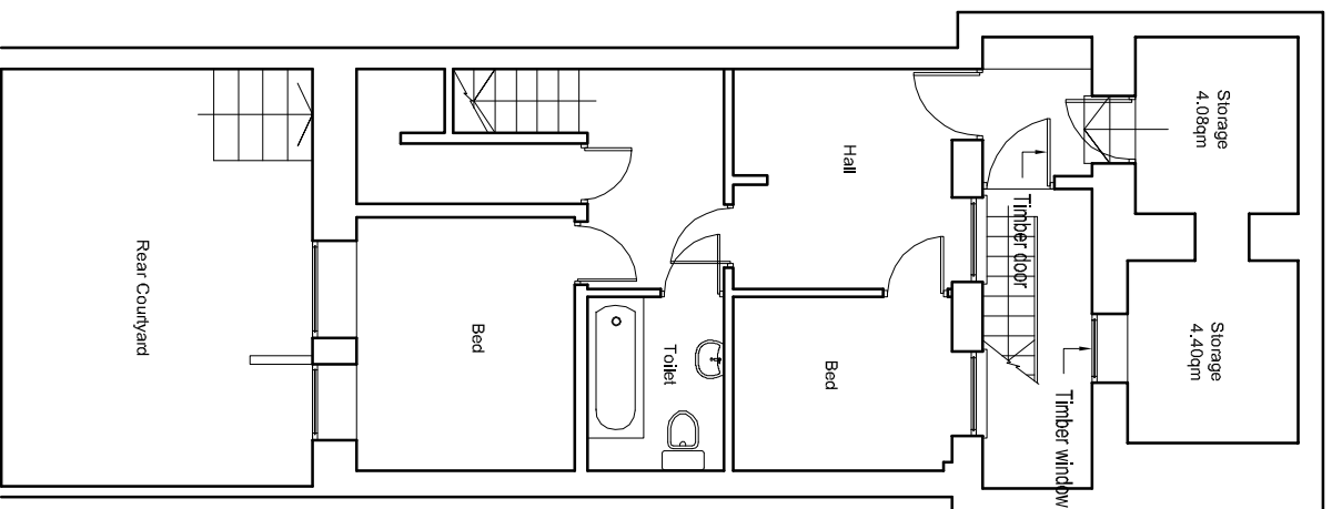
BASEMENT FLOOR PLAN PRIOR TO THE REAR EXTENSION
