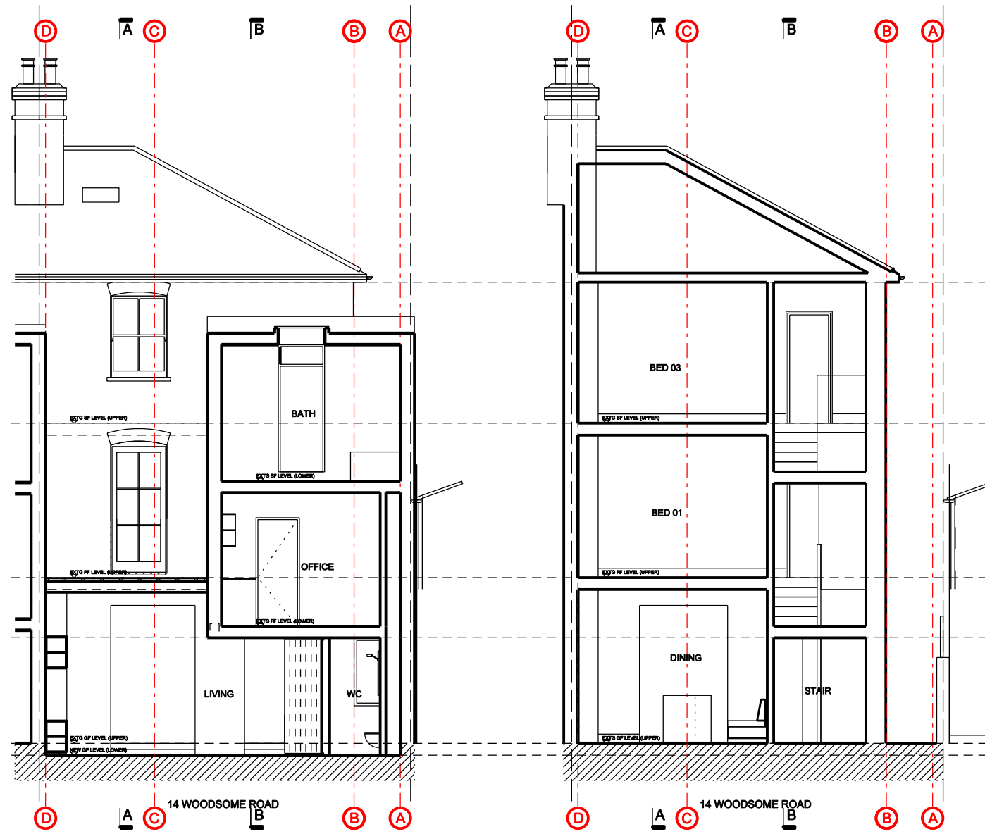
01 PROPOSED SECTION CC SCALE 1:100 AT A3
