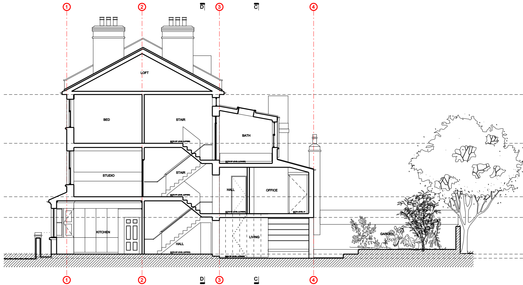
01 PROPOSED SECTION BB SCALE 1:100 AT A3
