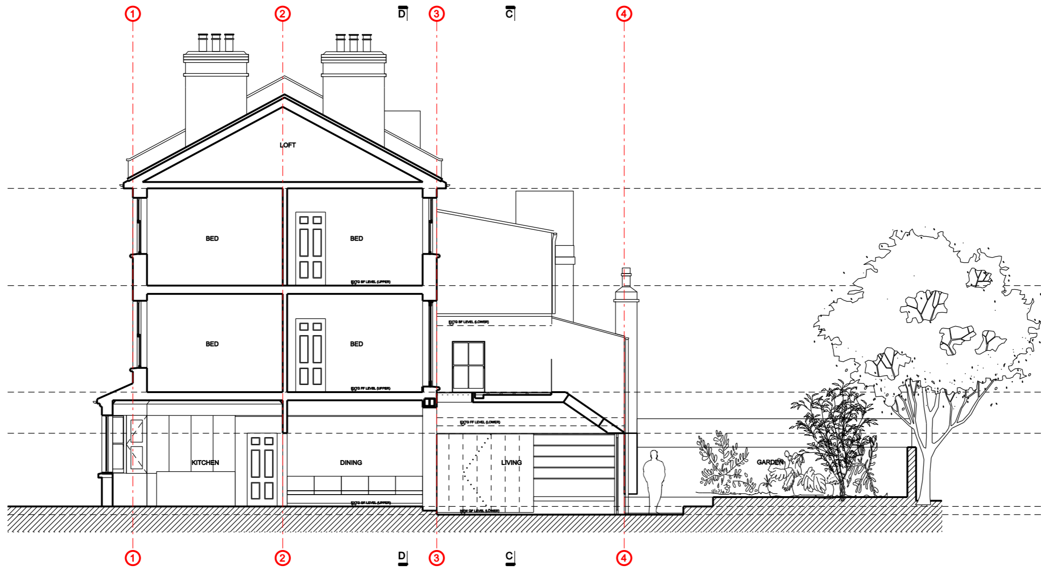
01 PROPOSED SECTION AA SCALE 1:100 AT A3
