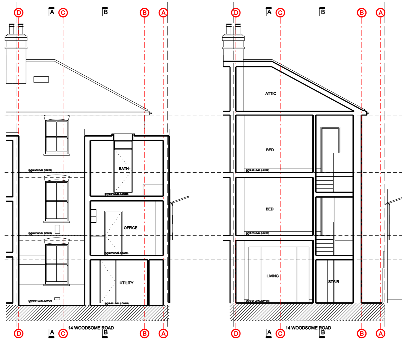
01 EXISTING SECTION CC SCALE 1:100 AT A3
